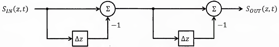
Figure 4. Double delay line canceler
