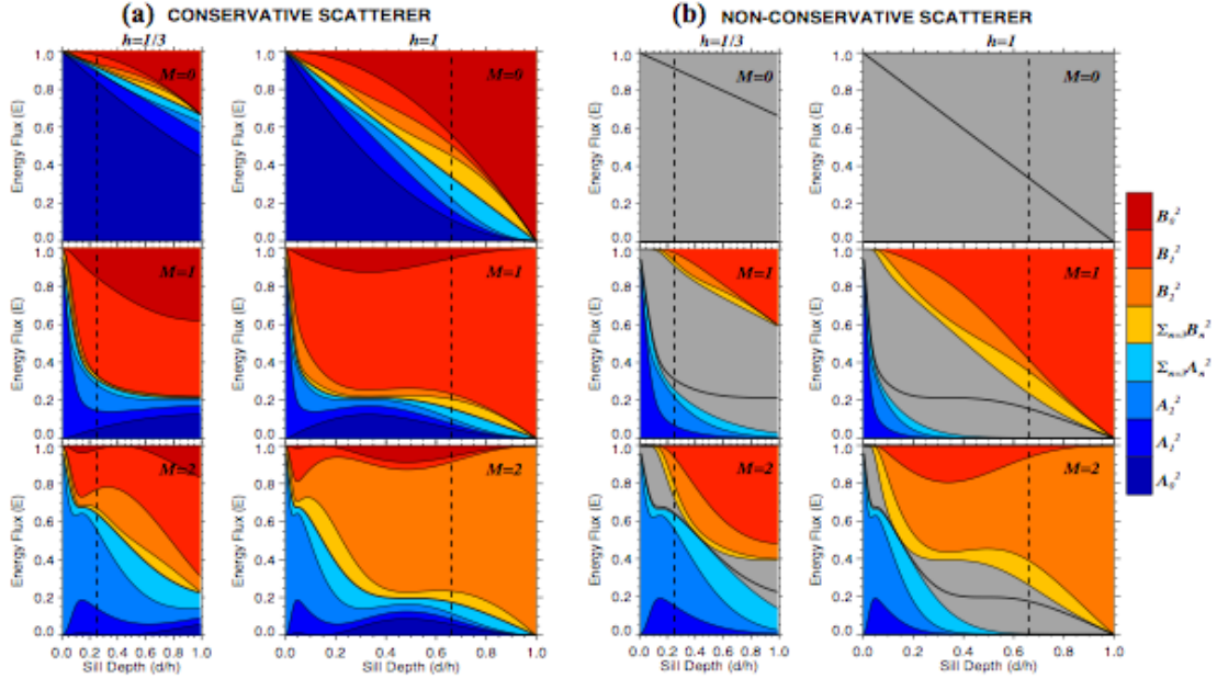
Fig. 1: Transmitted energy fluxes for (a) conservative scatterer, and (b) non-conservative scatterer, as function of sill depth relative to adjacent basin depth ( d/h ) for adjacent to incident basin depth ratios of h=1/3 (left) and h=1 (right). From top to bottom for incident CKW normal modes M=0,1,2 , where baroclinic normal mode structure is surface-trapped as found in tropical oceans. Energy flux transmitted by given normal mode is square of its transmission coefficient. Blue shades denote contributions to flux transmitted across gap ( A_n^2, n=0,1,2,\dots ), red shades to flux transmitted through gap ( B_n^2, n=0,1,2,\dots ); key is given on righthandside of plot. Total energy flux dissipated shaded grey. Dashed line on lefthandside plots denotes ratio appropriate to Lombok Strait and on righthandside plots to Timor Strait for CKWs incident from east Indian Ocean.
