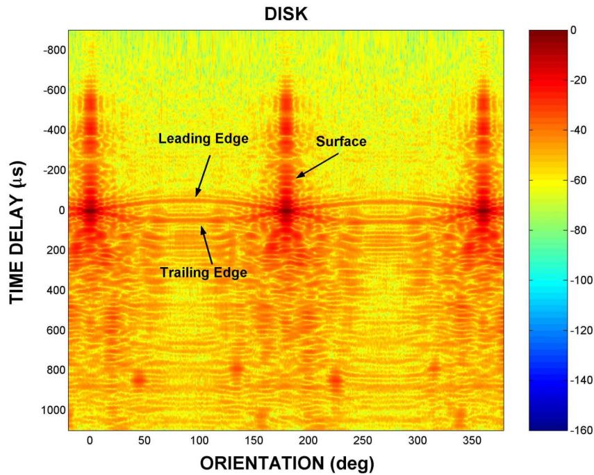
1. Color contour of compressed pulse output (dB) of acoustic backscattering versus orientation angle and time of return by 8-cm-diameter aluminum disk. Acoustic diffraction from leading and trailing edges of disk is illustrated.
