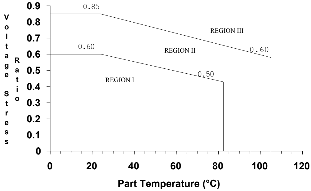
Figure 1-1 Glass, Porcelain (CYR), Mica (CMS)
