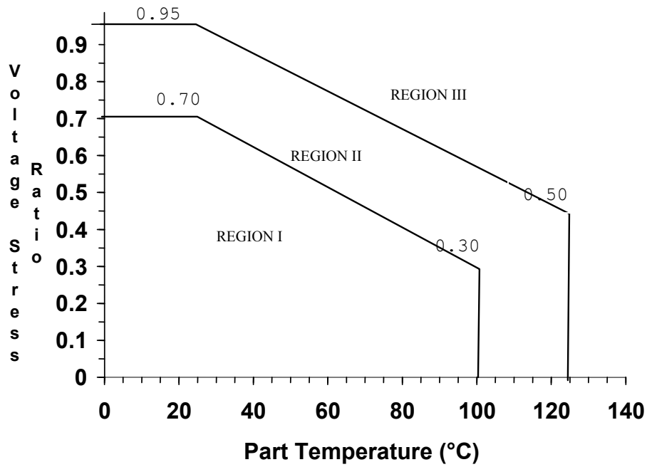
Figure 1-3 Solid Tantalum (CSR, CSS, CWR)
