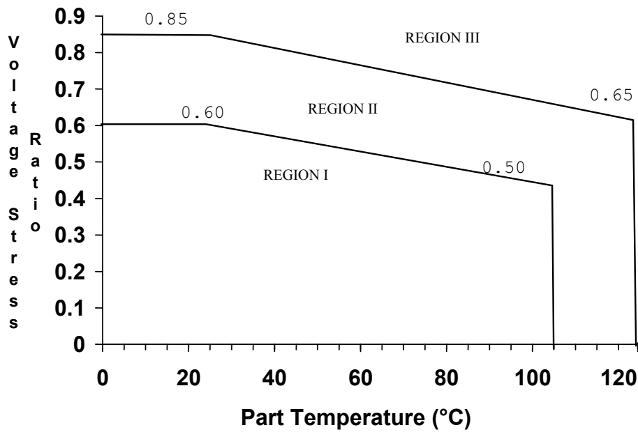
Figure 1-4 Wet Tantalum (CLR 79)
