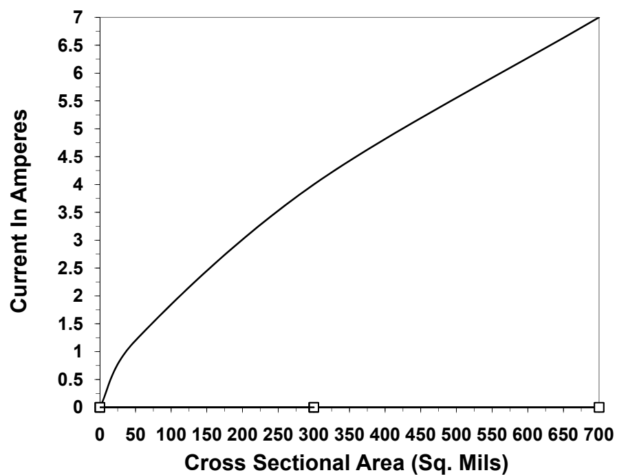
Figure 10-1 Conductor Current vs. Cross Sectional Area - Full
