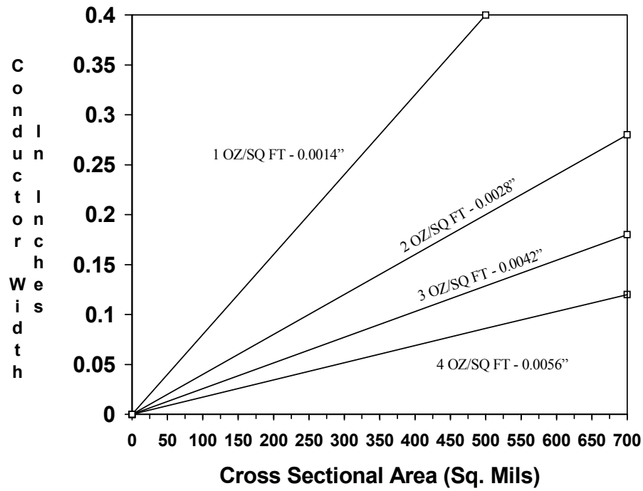
Figure 10-2 Conductor Width vs. Cross Sectional Area
