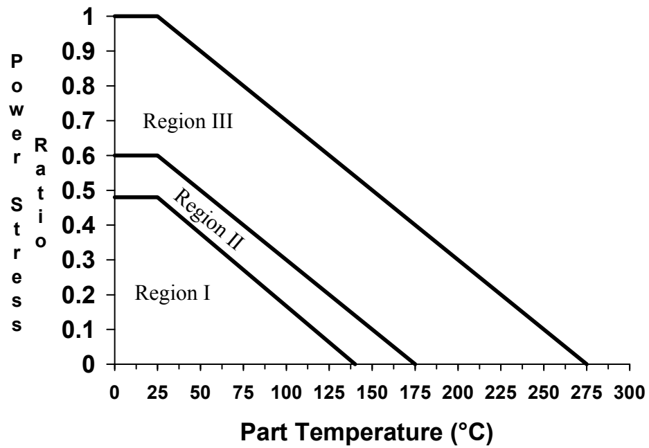
Figure 12-5 Wire Wound Power Resistor (RWR, RER)
