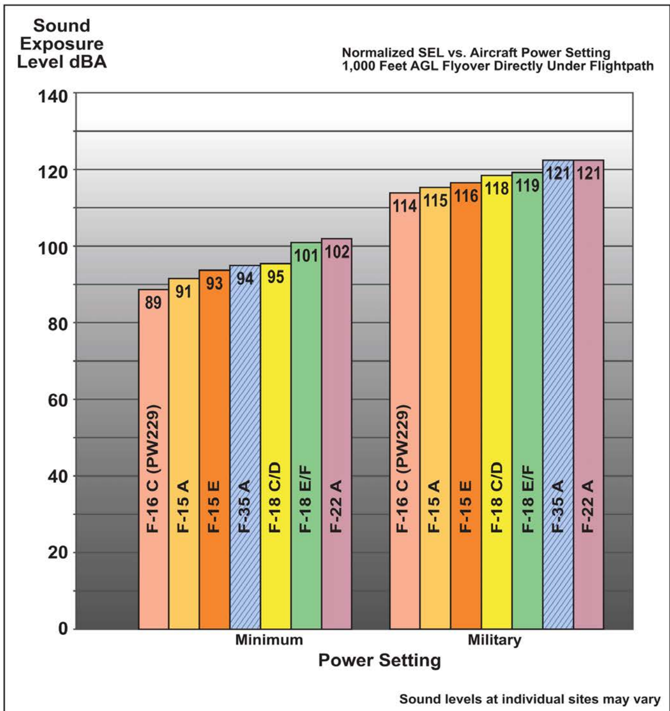
Figure 3.3-2 SEL for Various Aircraft
