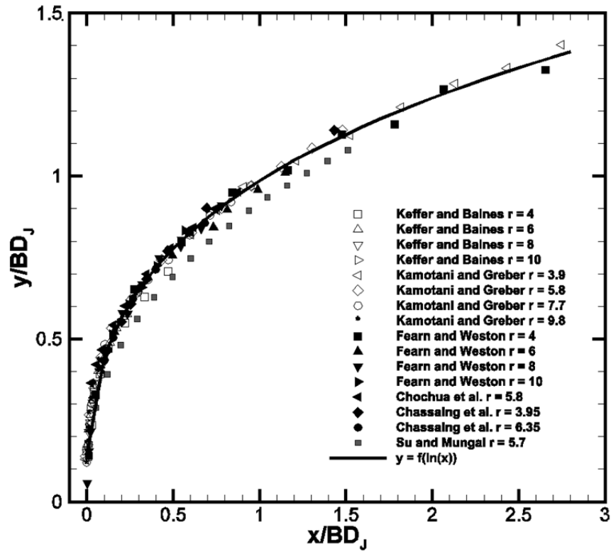
Figure 3: Unconfined transverse jet trajectories scaled with BD_j .
