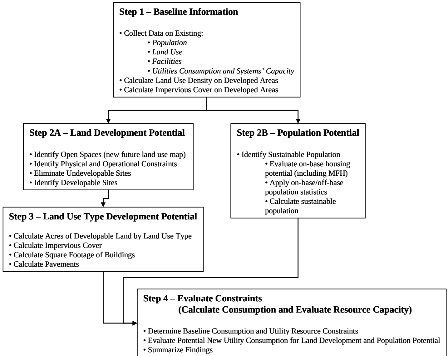
Figure 2.1-1. Non-Flying Mission Capability Analysis Process Flow Diagram
