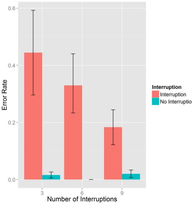
Figure 3. The average proportion of errors by number of interruptions at the PCS. Error bars are 95% confidence intervals.
