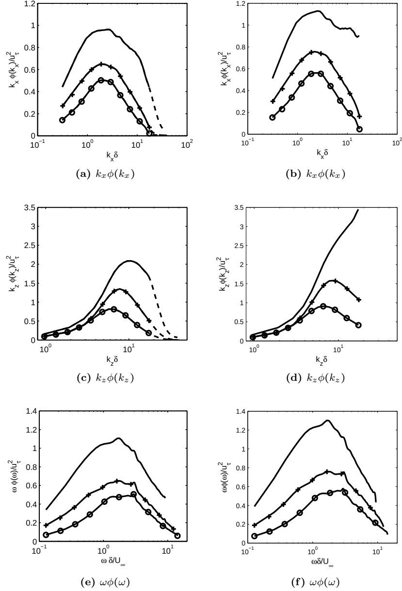
Figure 28: 1D premultiplied streamwise velocity spectra over (a,b): streamwise wavenumber, (c,d): spanwise wavenumbers, and (e,f): frequency where the lines are in all cases \text{---} : y^+ = 34 , \text{---+---} : y^+ = 108 , \text{---o---} : y^+ = 278 . The uncorrected data is shown in the left column and the corrected data is in the right column. For the uncorrected data, the dashed lines indicate data beyond the imposed cutoff, k_{cut} , beyond which the data begins to be attenuated
