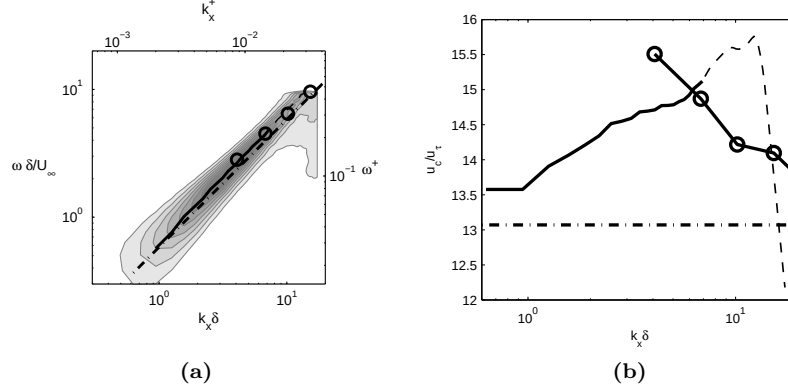
Figure 31: (a): The convection velocity calculated by finding the line of local maxima along k_x\omega\Phi(k_x, \omega) at y^+ = 34 is indicated by the solid black line (dashed black line beyond the point where noise influences the calculation) and displayed on top of the spectrum where the contours represent 20% to 80% of the maximum energy of the spectrum moving from light to dark shades in 10% increments. The dash-dot line indicates where \omega = \bar{U}k_x signifying a convection velocity equal to the local mean. The four open circles are data from Krogstad et al. [1998] at the same y^+ and similar Reynolds number. This data was converted from its original form, convection velocity plotted against streamwise probe separation, by converting the separation to a wavenumber and using the convection velocity for each wavenumber to define an associated frequency. (b): The convection velocity is plotted as a function of wavenumber where the lines and symbols are the same as in (a)
