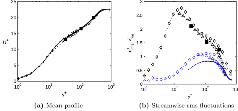
Figure 25: In (a): the mean velocity profile is presented where the symbols are \text{---} : Mean profile from wall normal measurements, \blacksquare : mean velocity from wall parallel plane measurements, \text{---} : Spalding fit [Spalding, 1961], \text{---+} : data from DeGraaff and Eaton [2000] at Re_\theta = 1430 , and \circ : points selected to represent the log layer. In (b): black lines and symbols are for u_{rms}^+ and blue lines and symbols are for v_{rms}^+ where, \blacksquare : u_{rms}^+ from wall parallel plane measurements, \bullet : v_{rms}^+ from the wall normal plane measurement, \text{---}\diamond\text{---} : data from DeGraaff and Eaton [2000] at Re_\theta = 1430 , and \text{---}\triangle\text{---} : data from Erm and Joubert [1991] at Re_\theta = 1003
