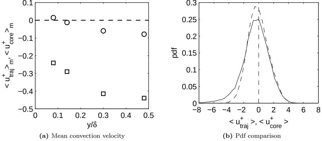
Figure 45: (a): Mean convection velocity for each plane where \square : \langle u_{traj} \rangle_m and \circ : \langle u_{core} \rangle_m . (b): Comparison of convection velocity pdfs for plane 3. Dashed line: \langle u_{core} \rangle , solid line: \langle u_{traj} \rangle
