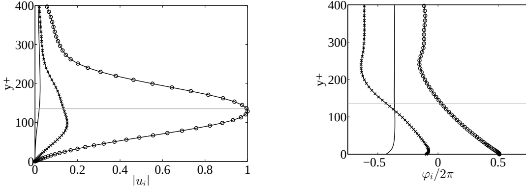
Figure 19: Wall-normal variation of (a) amplitudes of the three velocity components and (b) corresponding phases in multiples of 2\pi for the VLSM response mode with K = (1, 10, 2/3) at R^+ = 1800 . The lines denote -o- : u , -: v , - \times - : w . Solid/dashed horizontal line shows the location of the critical layer.
