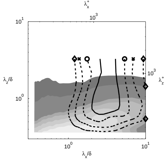
Figure 35: The contour lines represent the convection velocity at y^+ = 34 using the method outlined in Equation 28 where solid contours denote a convection velocity equal to the local mean and dotted contours with symbols are convection velocities below the local mean with o: \bar{U}^+ - u_\tau , x: \bar{U}^+ - 2u_\tau , and \diamond : \bar{U}^+ - 3u_\tau . The shaded contours represent 20 to 80% of the maximum energy of k_x k_z \Phi(k_x, k_z) in 10% increments moving from light to the dark shades
