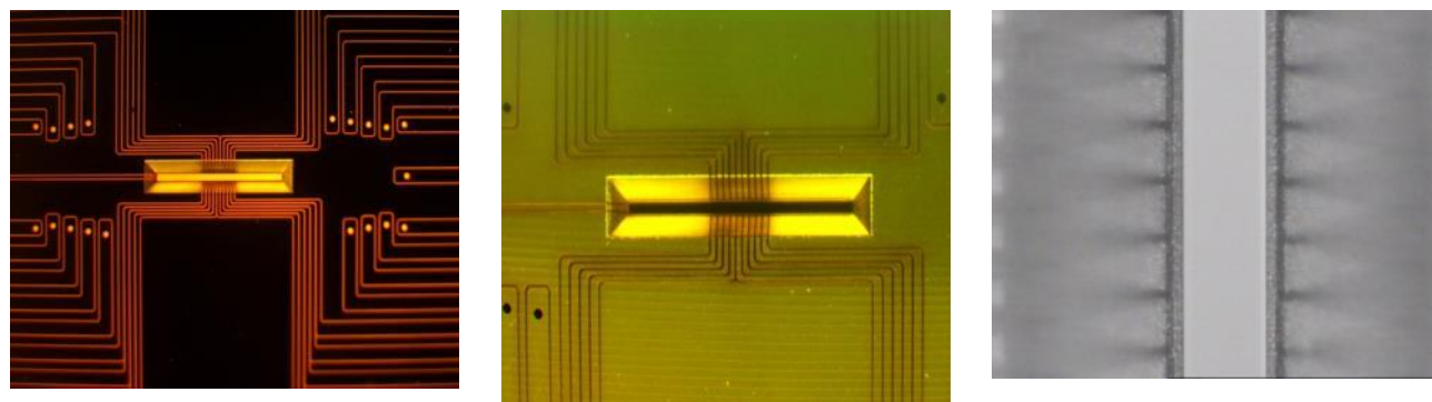
Figure 16: Microscope images of the top surface of a microtrap with electrical vias. The trap platform consists of a 100 \mu\text{m} wide, 2.4 mm long and 100 \mu\text{m} deep slot centered in a 500 \mu\text{m} thick silica substrate. The slot is recessed through 45° angled surfaces. The vias seen in the left and center images electrically connect the corresponding top surface electrodes to the bottom surface DC control electrode array. The electrodes are separated by a 10 \mu\text{m} gap and patterned through laser ablation of the Au/Cr coating.
