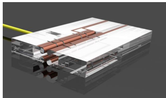
Figure 26: Linear Paul Trap. (Left) Model showing the rod geometry. (Right) Test piece with two sets of rods positioned side-by-side. This demonstrator was fabricated in a 500-micron thick fused silica blank. The length of the rod is approximately 10-mm.
