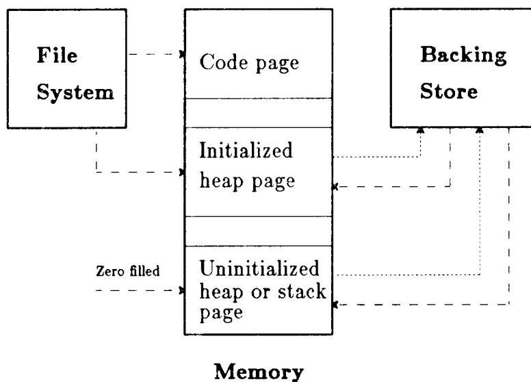
Figure 8. Lifetime of a Sprite page. Code pages live in two places, the file system and memory. Code pages never have to live on backing store because they are never modified. Initialized data pages live in the file system and memory until they get modified, and then spend the rest of their life in memory and backing store. Uninitialized heap and stack pages are filled with zeroes initially and then spend the rest of their life in memory and backing store.
