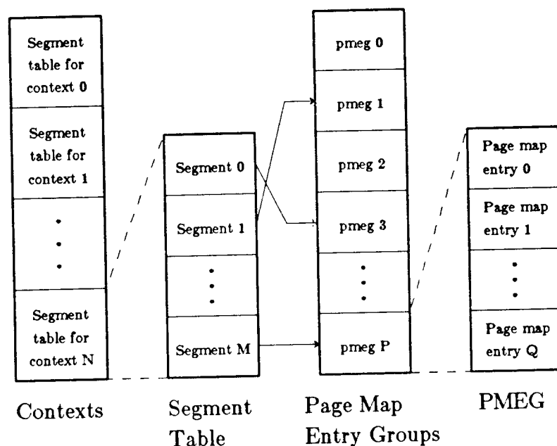
Figure 10. The Sun-2 memory mapping mechanism. The values for N, M, P and Q on a Sun-2 are 8, 512, 256, and 16 respectively. The Sun-3 architecture uses the same memory mapping mechanism as a Sun-2 with the exception that M is equal to 2048.
