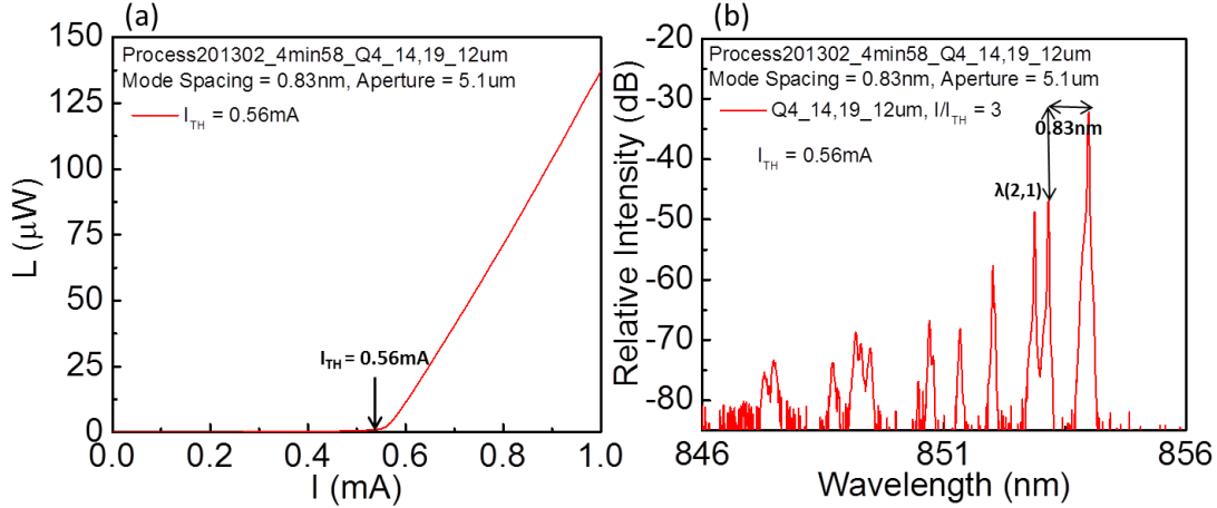
Figure 4: The (a) L-I and (b) Spectrum characteristics of the device under test. The laser threshold current, I_{TH} , of the device is 0.56\text{mA} . The mode spacing between the fundamental mode, \lambda(1, 1) , to the first second-order mode, \lambda(2, 1) , is 0.83\text{nm} which corresponds to an optical aperture opening of 5.1\mu\text{m}^4 .
