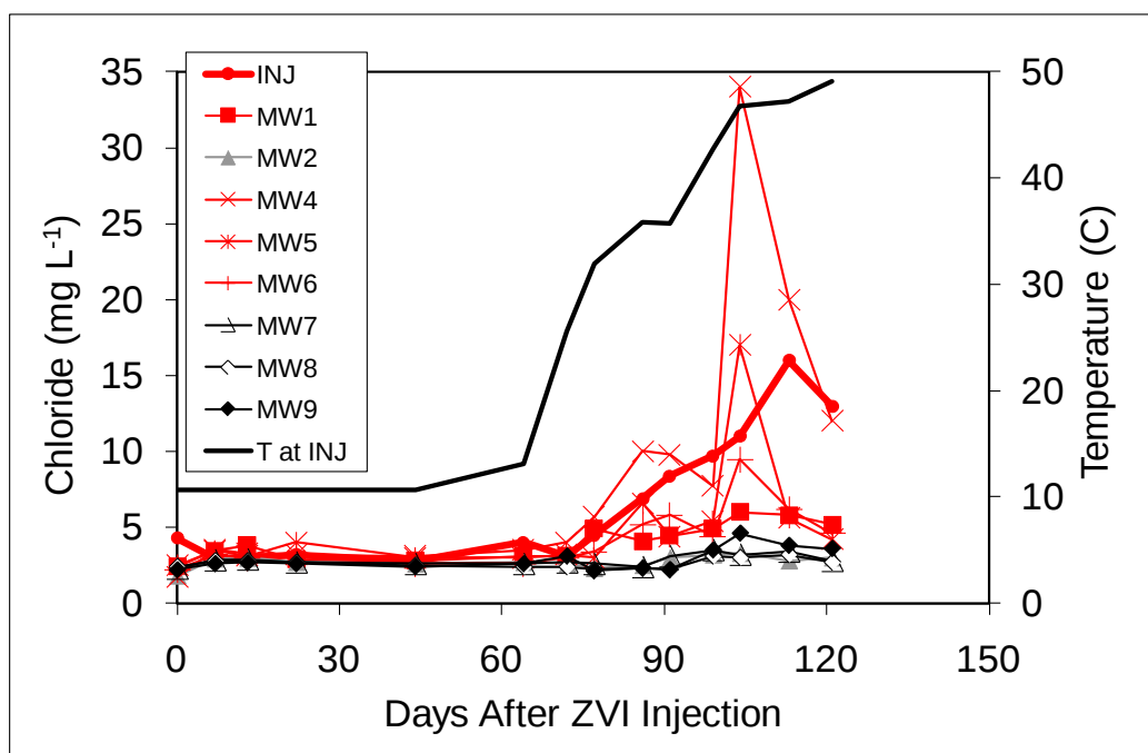
Figure 17. Chloride concentration over time in the ZVI test cell.
