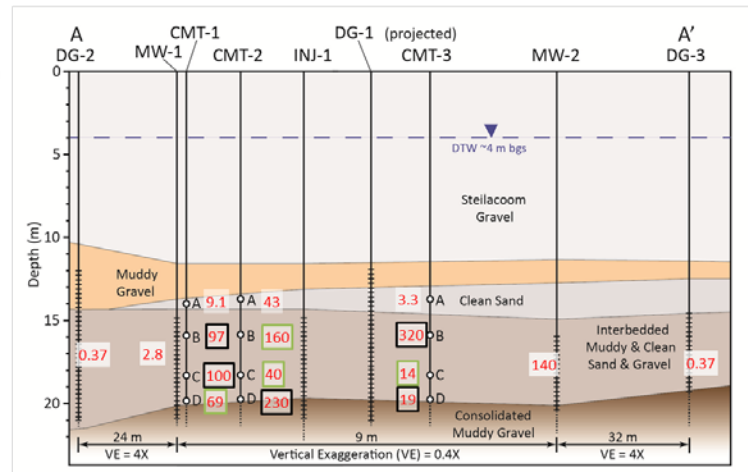
Figure 22. Groundwater sampling results from performance monitoring – 8 months post injection.
