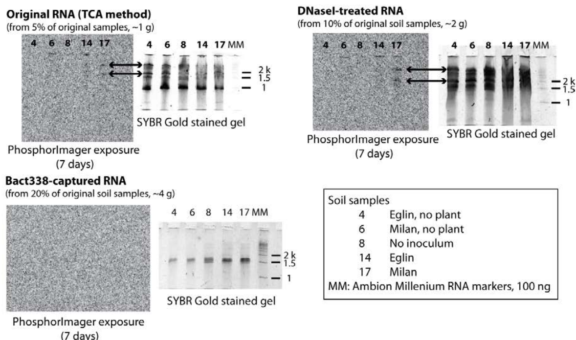
Figure 31. Incorporation of ^{14}\text{C} -bicarbonate into soil microbial RNA.
