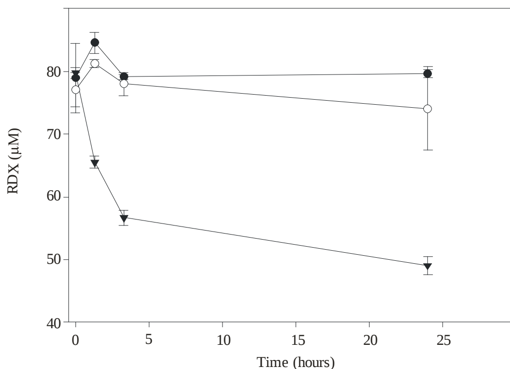
Figure 21. Uptake of RDX by P. fluorescens F113 containing pME6031- xplA . Cells were grown for 24 h at 30 °C and then transferred to minimal media containing RDX. Reactions were stopped by using the same volume of 10 % acetic acid (w/v). RDX-concentration was monitored by injecting an aliquot onto an 18 C-column and separating using an isocratic gradient of 50:50 Methanol/Water. (▼) Pseudomonas fluorescens F113 transformed with pME6031- xplA , (○) P. fluorescens F113 containing the empty vector and (●) wild type P. fluorescens F113.
