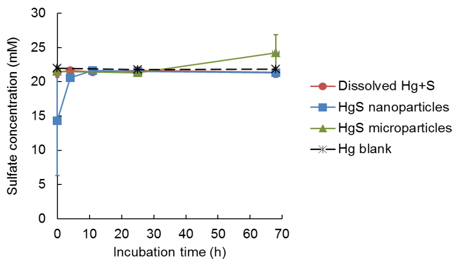
Figure S4. Sulfate concentrations in slurry microcosms exposed to 5 nmol g -1 (dw) dissolved Hg(NO 3 ) 2 and Na 2 S, HgS nanoparticles or HgS microparticles in Experiment 2. The slurries were prepared with sediments from (a) Site 1 and (b) Site 3. The error bars represent 1 s.d. for replicate samples (n=2-3) in the test groups. Single replicate of slurries were incubated for the Hg blank control.
