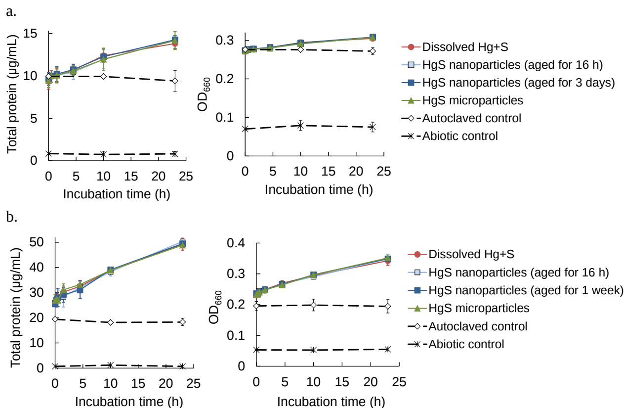
Figure 2.3. Bacterial growth in SRB cultures exposed to different forms of mercuric sulfides. Total protein content and optical density (OD 660 ) of (a) D. propionicus 1pr3 cultures and (b) D. desulfuricans ND132 cultures.
