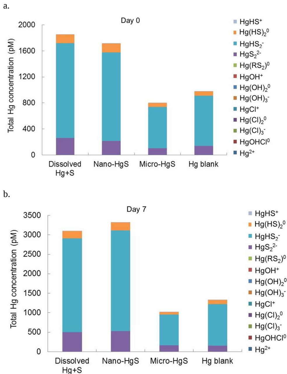
Figure S6. Speciation of dissolved Hg (i.e., total Hg remained in the aqueous phase after ultracentrifugation at 370,000 g for 1 h) in sediment slurries amended with 2 nmol \text{g}^{-1} (dw) (345 nmol Hg per L of water was added into the slurries) dissolved \text{Hg}(\text{NO}_3)_2 and \text{Na}_2\text{S} , HgS nanoparticles or HgS microparticles in Experiment 1. The slurries were prepared with sediments from Site 3. Samples were collected immediately (a) and 7 days (b) after mercury amendments. ‘Hg blank’ represents slurries without mercury addition.
