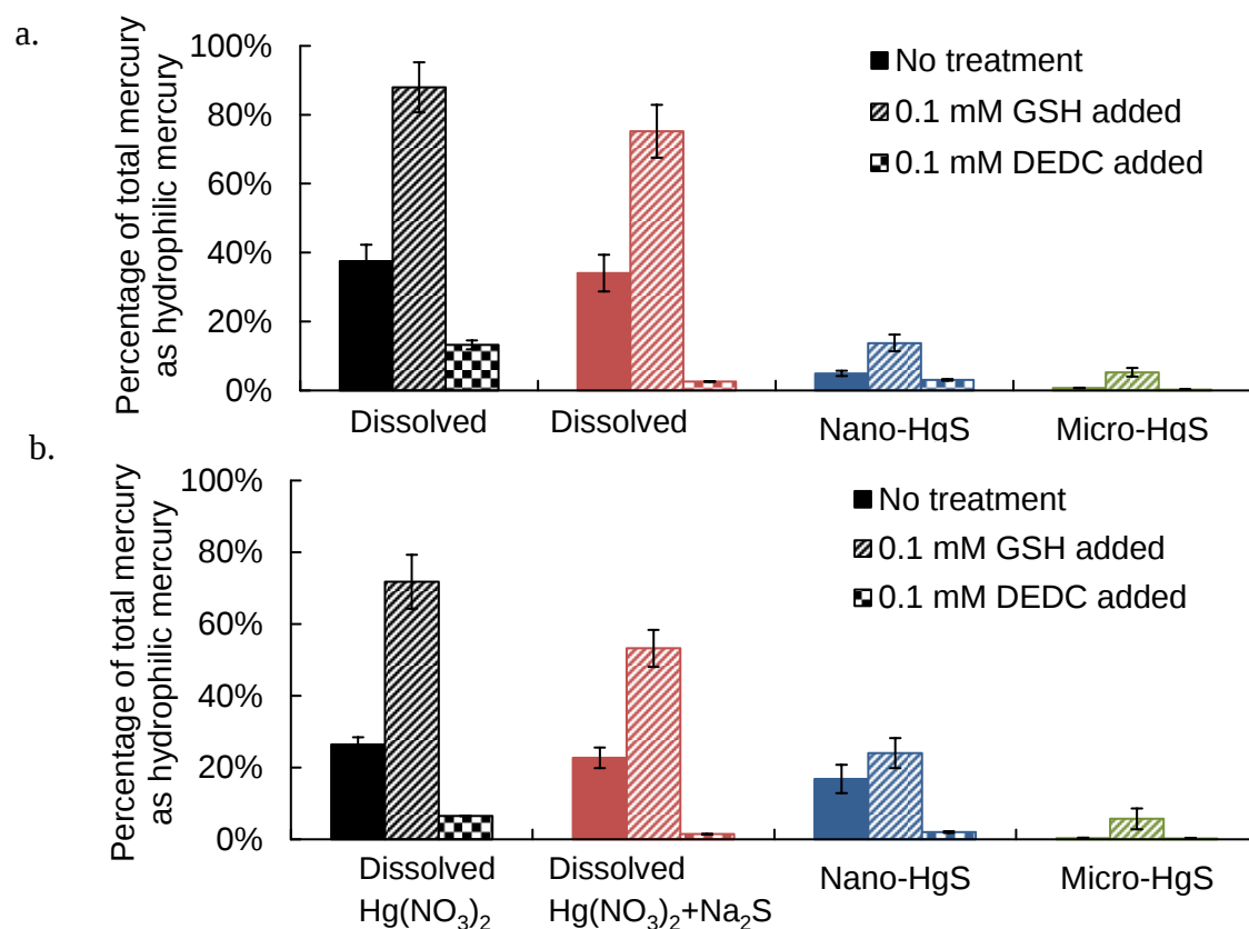
Figure 2.13. Hydrophilic mercury in HgS-amended media after competitive ligand exchange with GSH or DEDC and C 18 solid-phase extraction. Uninoculated medium solutions (for culturing D. propionicus 1pr3) were spiked with 1 nM dissolved Hg(NO 3 ) 2 , 1 nM dissolved Hg(NO 3 ) 2 and Na 2 S, 1 nM humic-HgS nanoparticles (aged for 16 h), and 6 nM HgS microparticles. Ligand exchange reactions were performed by amending aliquots of these samples with GSH or DEDC at two time points after the mercury amendment: (a) Immediately (less than 10 min). (b) 23 h. GSH and DEDC were mixed in the samples for 1 h and then filtered through a C 18 resin. All solutions received the same humic acid concentration (0.2 µg-C/L). Error bars represent ±1 s.d. for duplicate samples.
