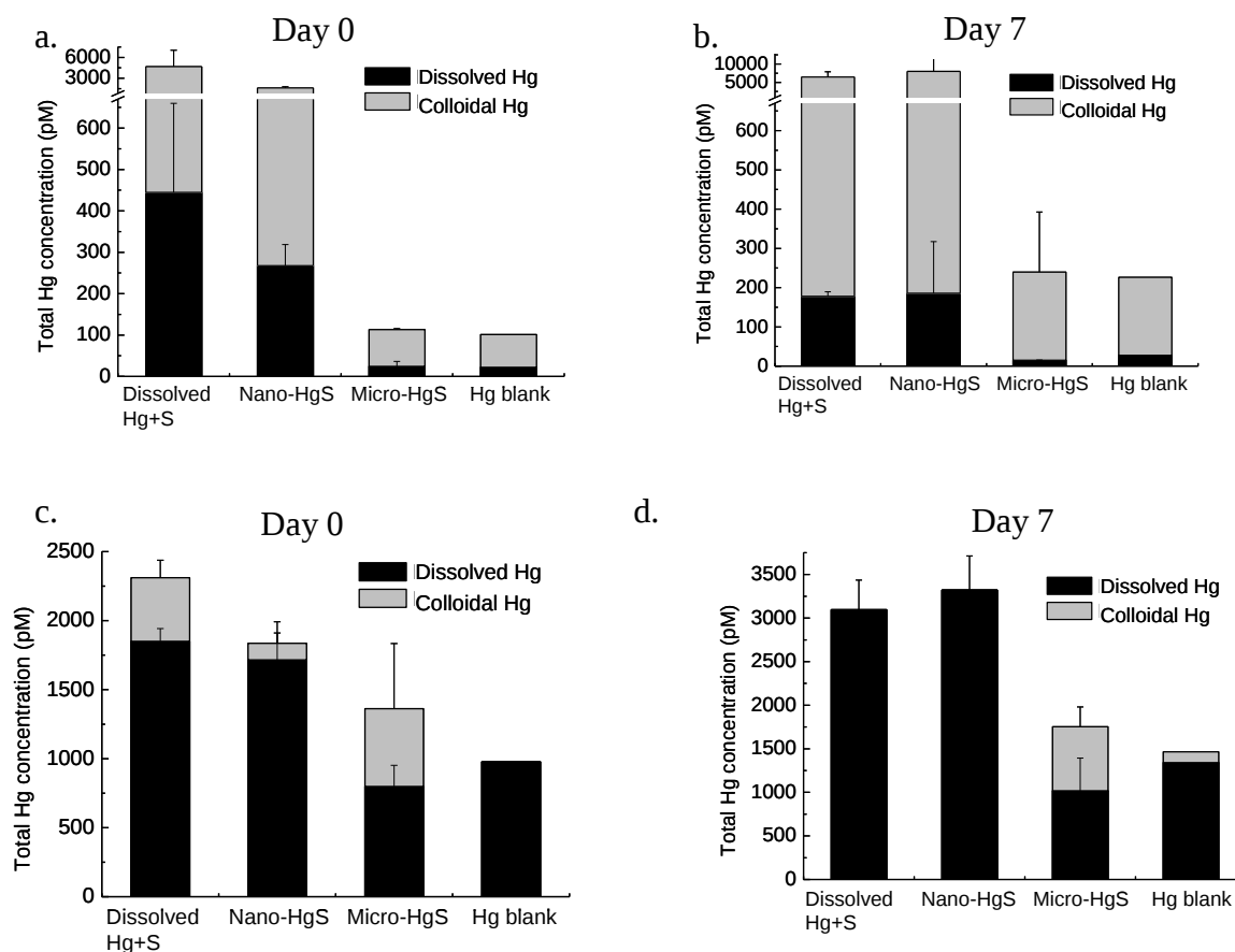
Figure 4.4. Hg fractionation in sediment slurries amended with 2 \text{ nmol g}^{-1} \text{ (dw)} added as dissolved \text{Hg}(\text{NO}_3)_2 and \text{Na}_2\text{S} , HgS nanoparticles or HgS microparticles in Experiment 1. This Hg spike corresponded to 345 \text{ nmol Hg per L} of water was added into the slurries. The slurries were prepared with sediments from Site 1 ( a and b ) and Site 3 ( c and d ). (Ultra) centrifugation was performed within 15 min ( a and c ) and 7 days ( b and d ) after mercury amendments. ‘Dissolved Hg’ represents the total Hg that remained in the supernatant after ultracentrifugation at 370,000 g for 1 h. ‘Colloidal Hg’ represents the concentration difference of supernatant Hg after centrifugation at 6,700 g for 5 min and ultracentrifugation at 370,000 g for 1 h. ‘Hg blank’ represents slurries without mercury addition. The error bars represent 1 s.d. for duplicate samples in the test groups. Single replicate of slurries were incubated for the Hg blank control.
