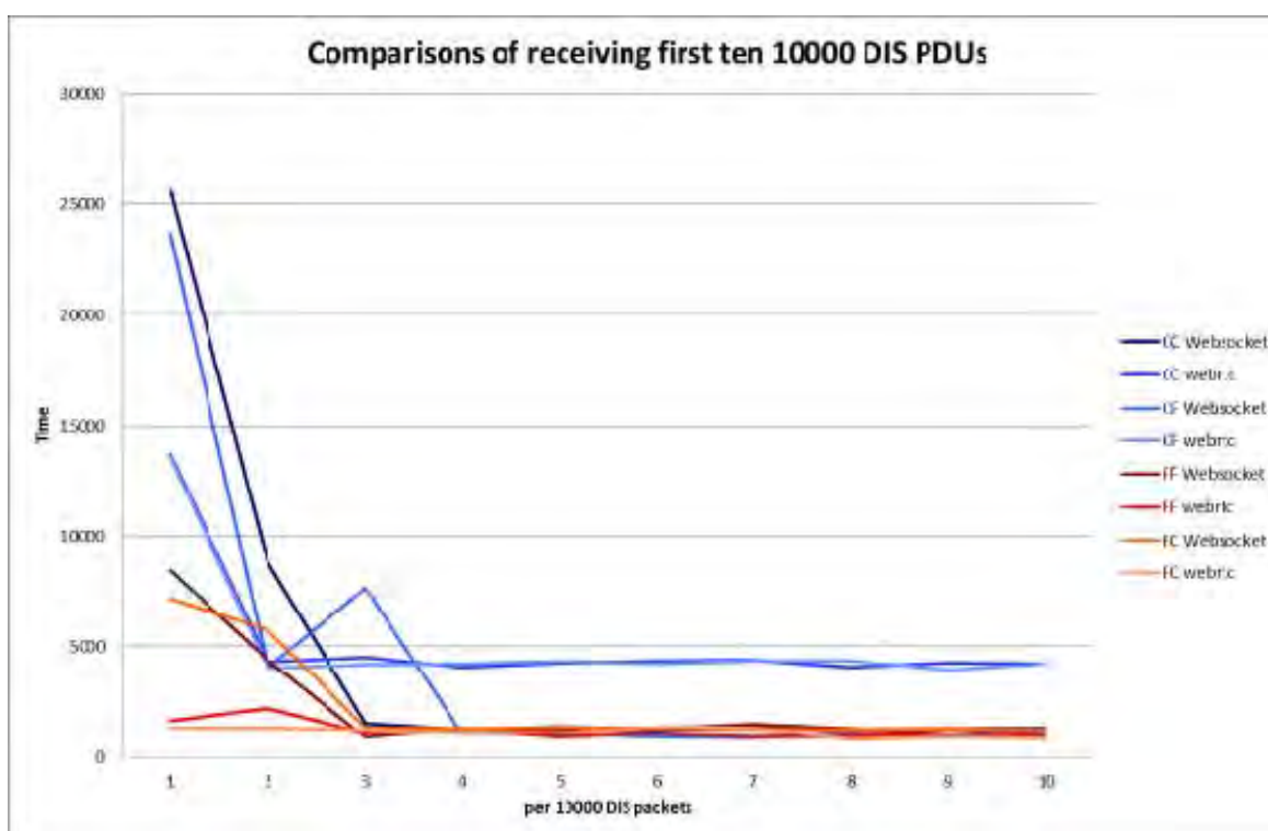
Figure 47. The comparisons of receiving first ten 10,000 DIS PDUs in the linear form.
