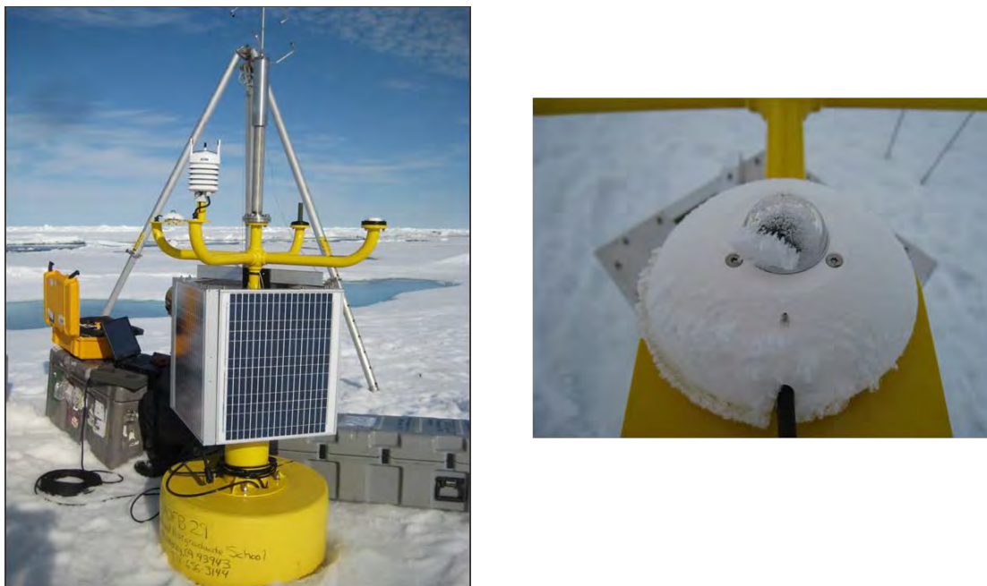
Figure 62. Photographs of AOFB 29 deployed in the Arctic in August 2014. Left Image: small domed solar sensor on the left-most arm of the meteorology tree collects shortwave (visible) surface solar intensity time series which can be used to understand the effects of varying solar intensity in the open water fraction/heat content relationship. Right Image: close up image of the solar sensor used to collect shortwave solar information (images courtesy Mr. Jim Stockel 2014).
