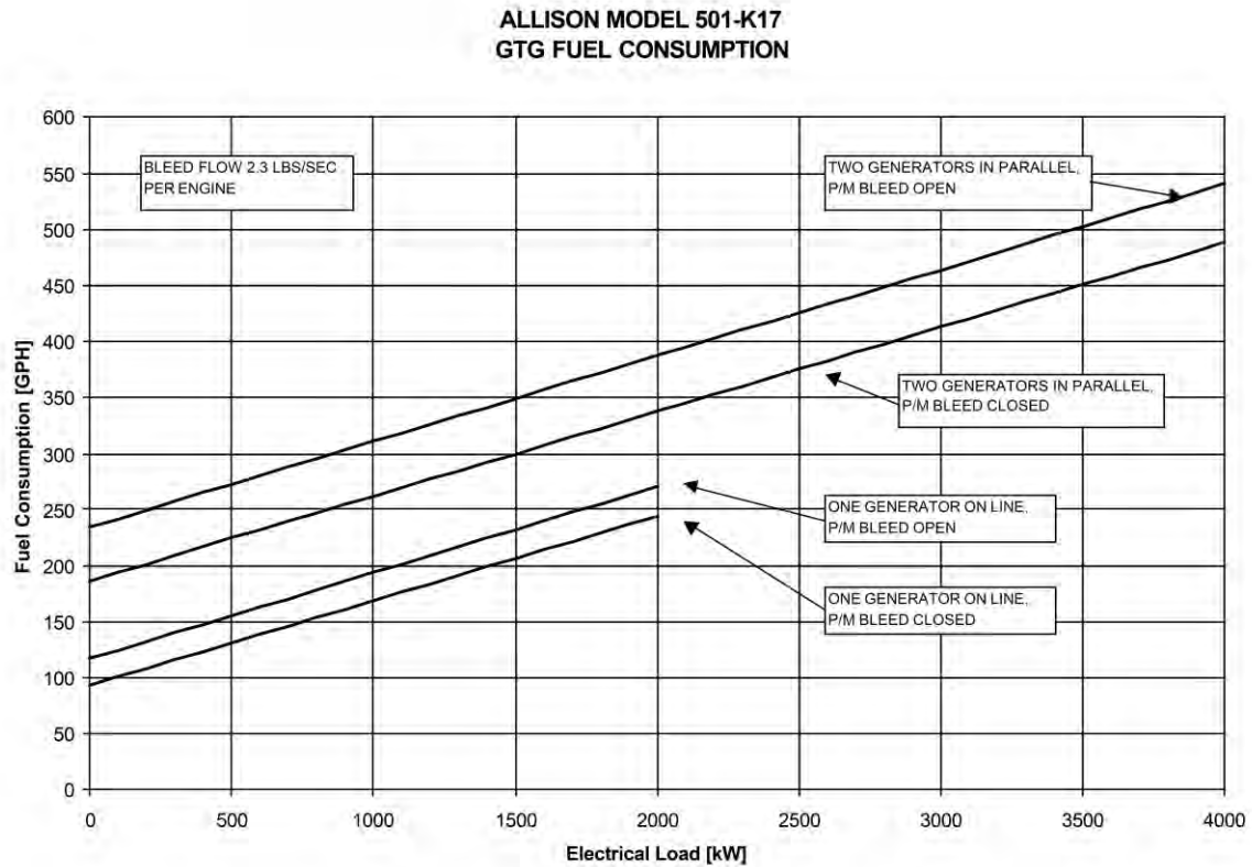
Figure 8. Fuel consumption of single-generator operations and two generators operated in parallel using Allison GTGs. These GTGs are used onboard Ticonderoga-class cruisers (from Bennett 2014). Approximately 95-120 GPH less fuel is burned when operating one GTG vice two.
