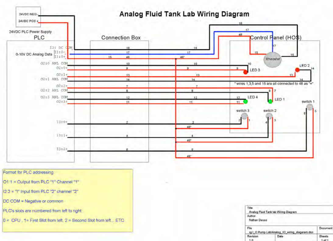
Figure B1. AFTL wiring diagram
