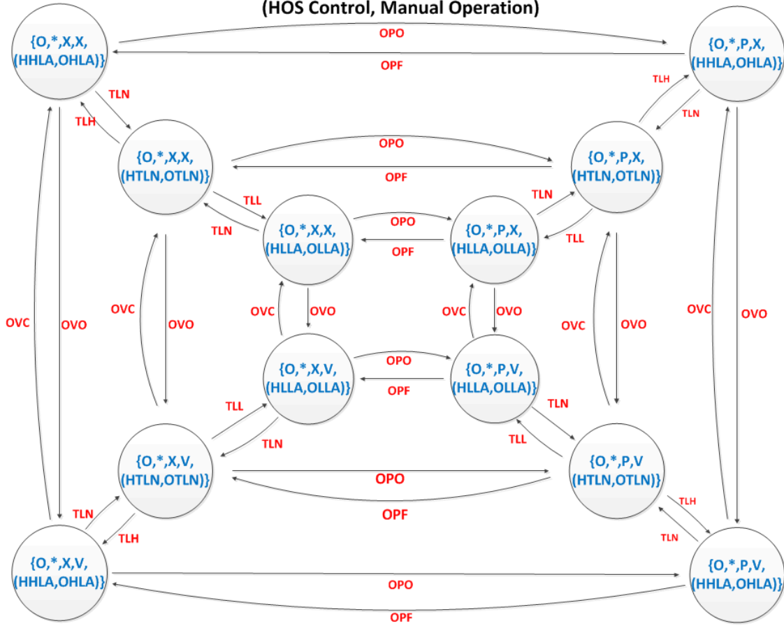
Figure D4. HOS-Manual and HOS-Auto state diagram.
