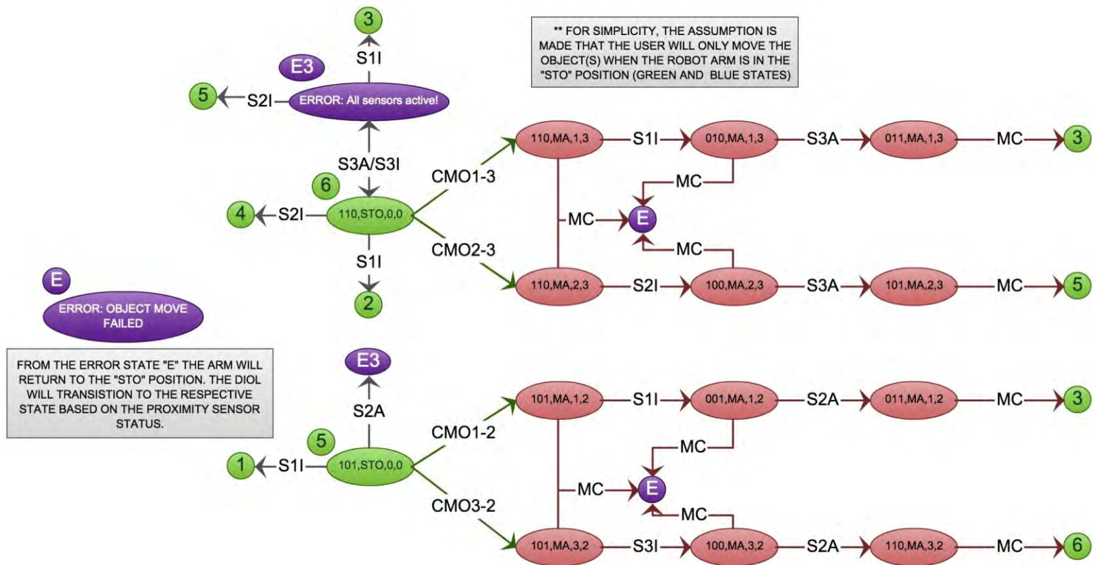
Figure E2. DIOL state diagram part 1 of 2
