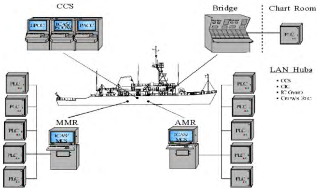
Figure 2. MCM-1 digital MCS system, from [14]
