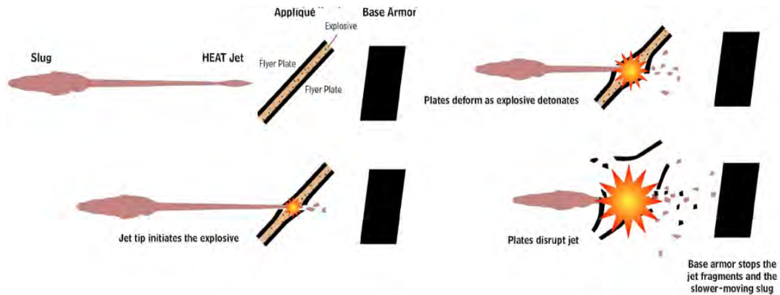
Figure 4. Mechanics of Explosive Reactive Armor (ERA) (from Kempinski and Murphy 2012).
