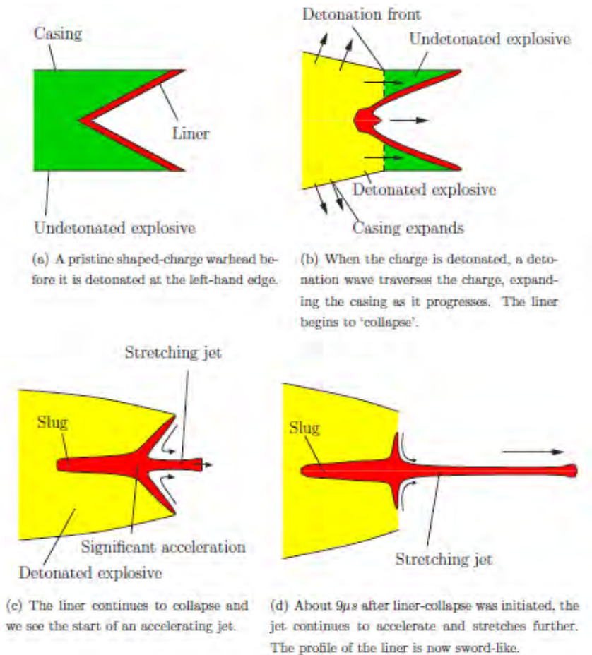
Figure 3. A Sequence of Events in Shaped-charge Jet Formation (from Poole 2005).
