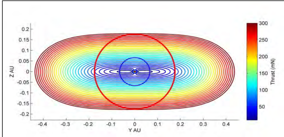
Figure 22. Equithrust contours of 1000 kg spacecraft around Mars (from Macdonald et al., 2011).
