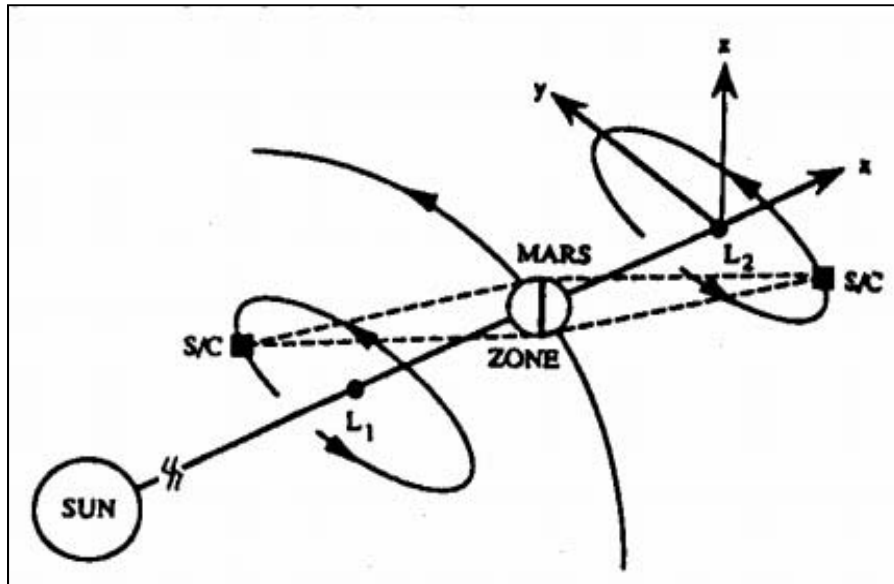
Figure 19. Sun-Mars L1 and L2 Lagrange orbits (from Strizzi et al., 2001)
