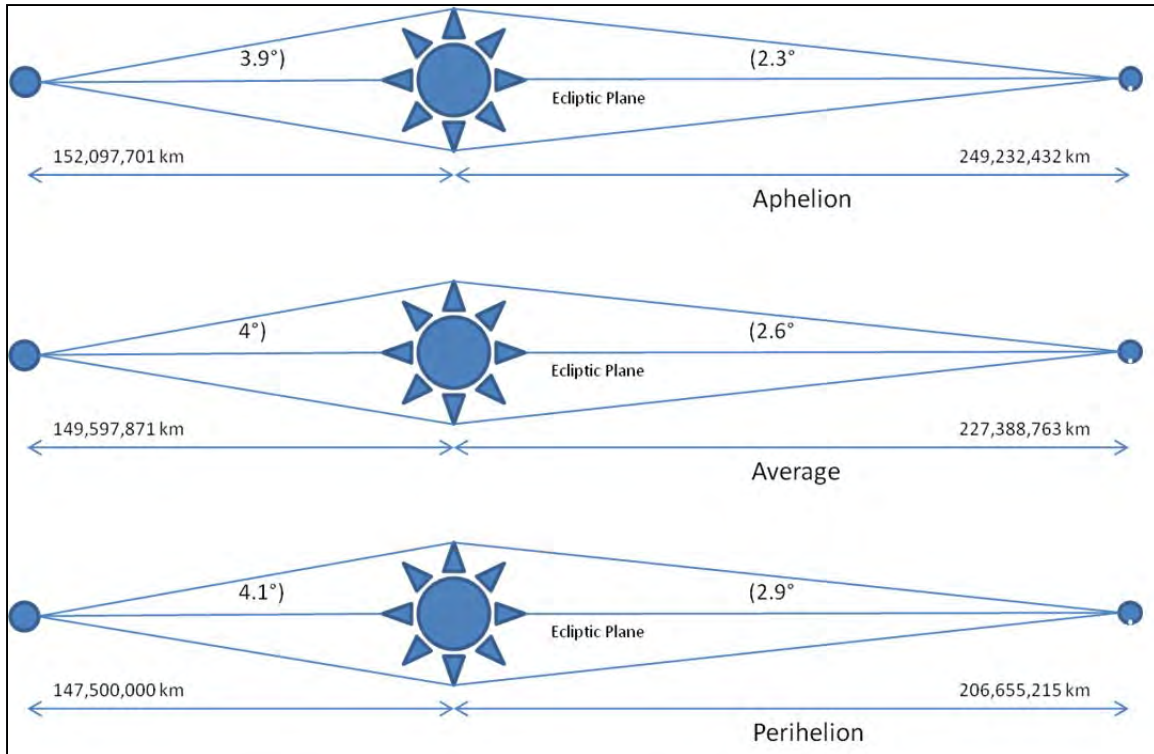
Figure 16. Solar occultation angles
