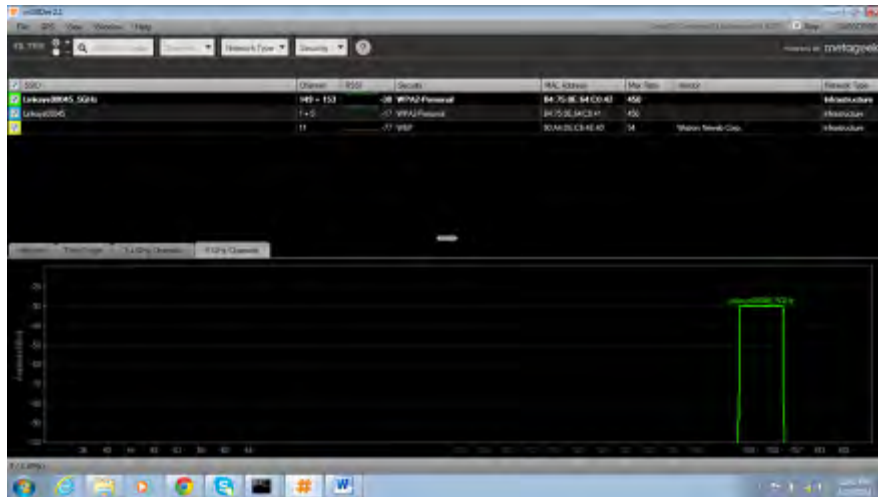
Figure 39. Spectrum survey using inSSIDer 2.1–5.8 GHz.
