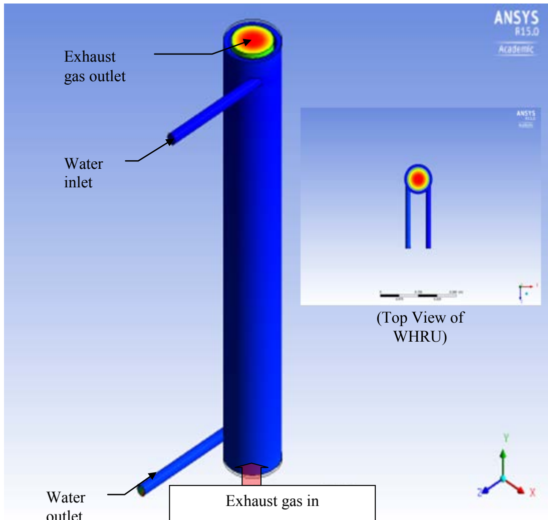
Figure 53. Isometric view (and top view) of CFD model with water placement Type 3 (water inlet and outlet located at x^* = \pm 0.8 from centerline and y/L = 0.1 from the top and bottom edges of WRU).
