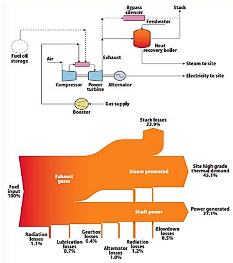
Figure 2. Layout of an typical exhaust gas WHRS used for combined heat and power (from CHP Focus, 2014)
