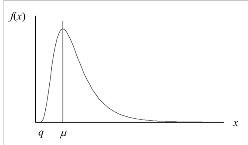
Figure 1-2. The Lognormal Distribution.
