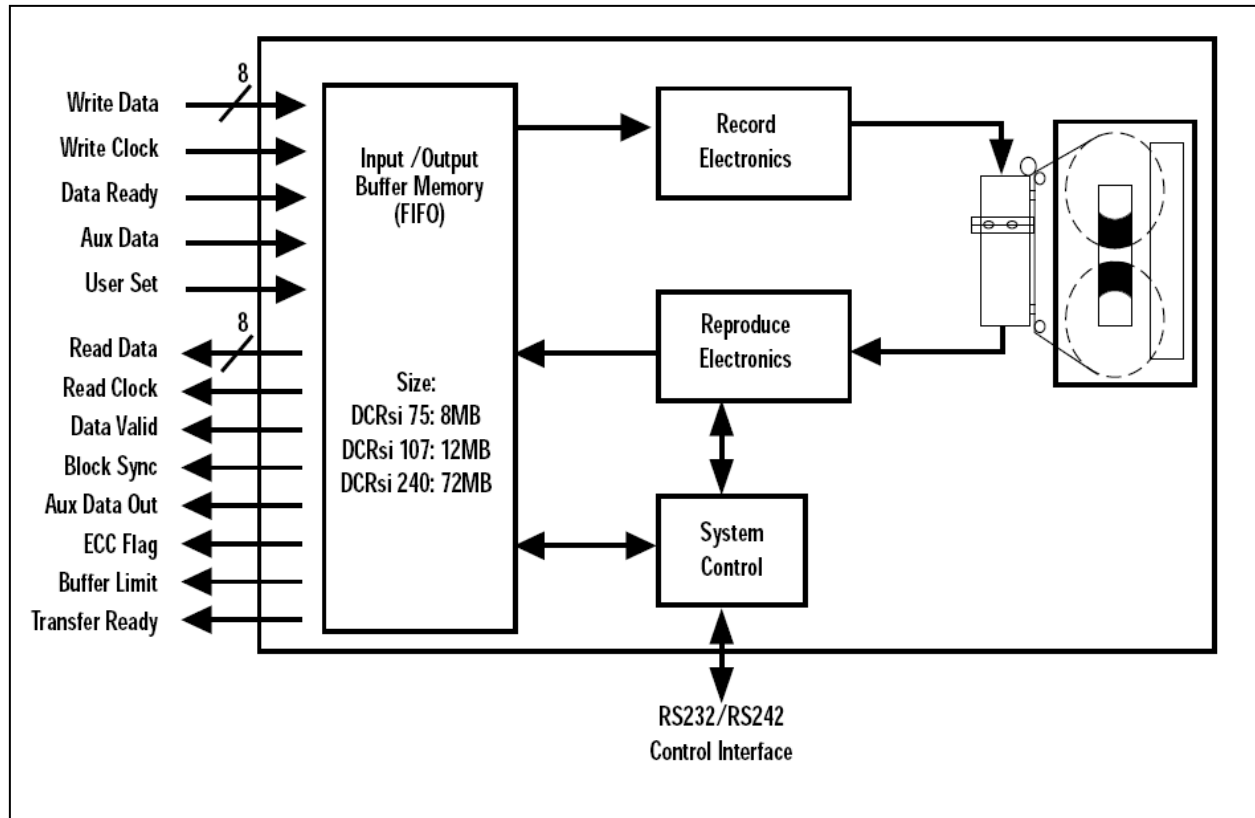
Figure 6-50. DCRsi interface.
