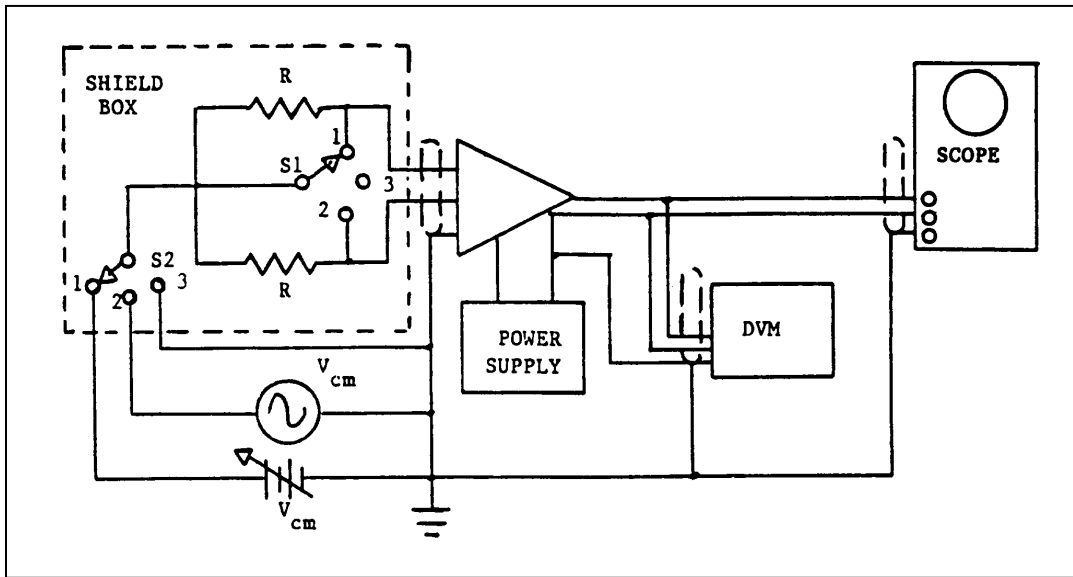
Figure 3-4. Block diagram for common mode rejection test.
