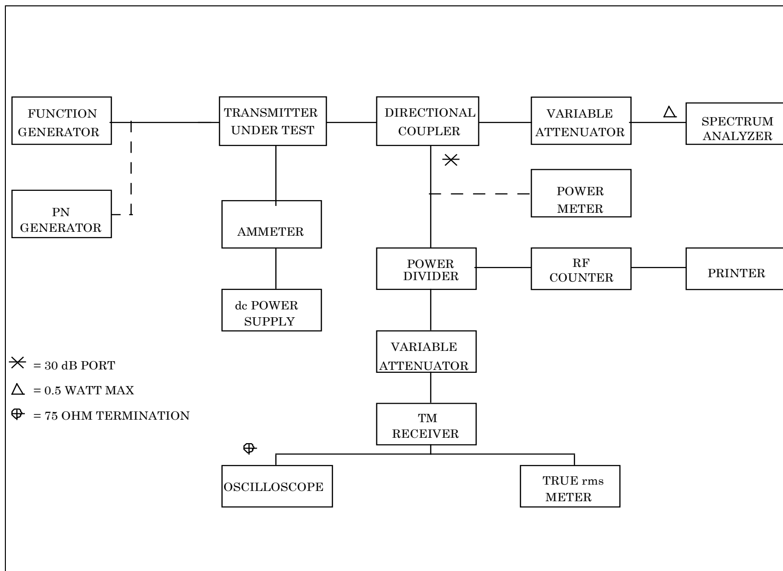
Figure 5-32. Premodulation filter test setup.
