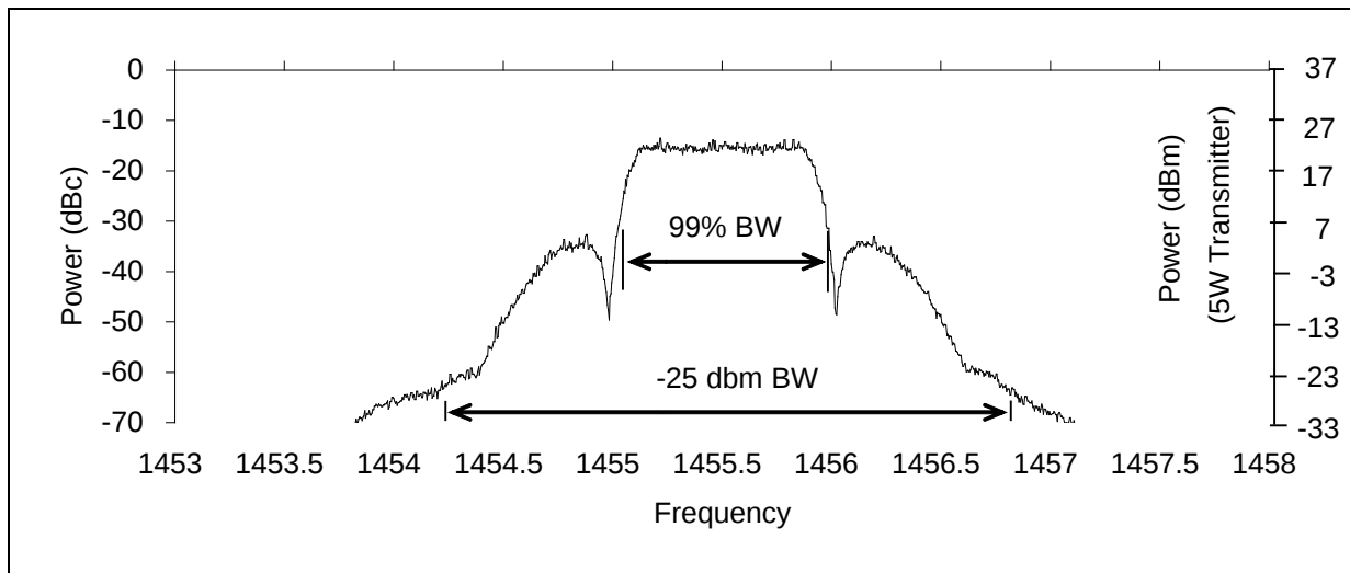
Figure 5-33. NRZ PCM/FM spectrum test.
