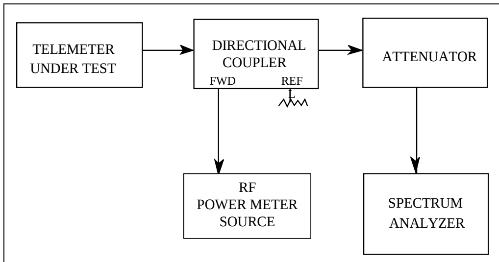
Figure 5-34. Laboratory setup.
