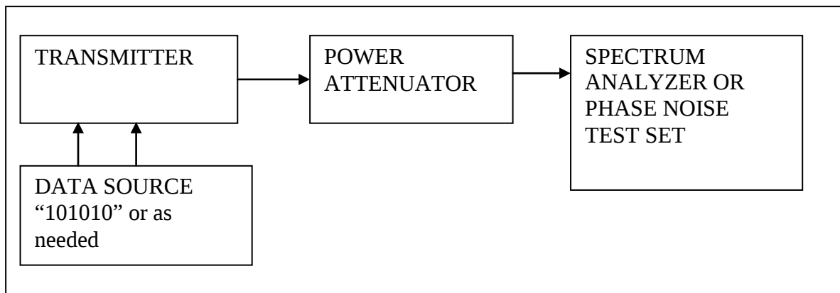
Figure 5-38. Test setup for transmitter phase noise test.
