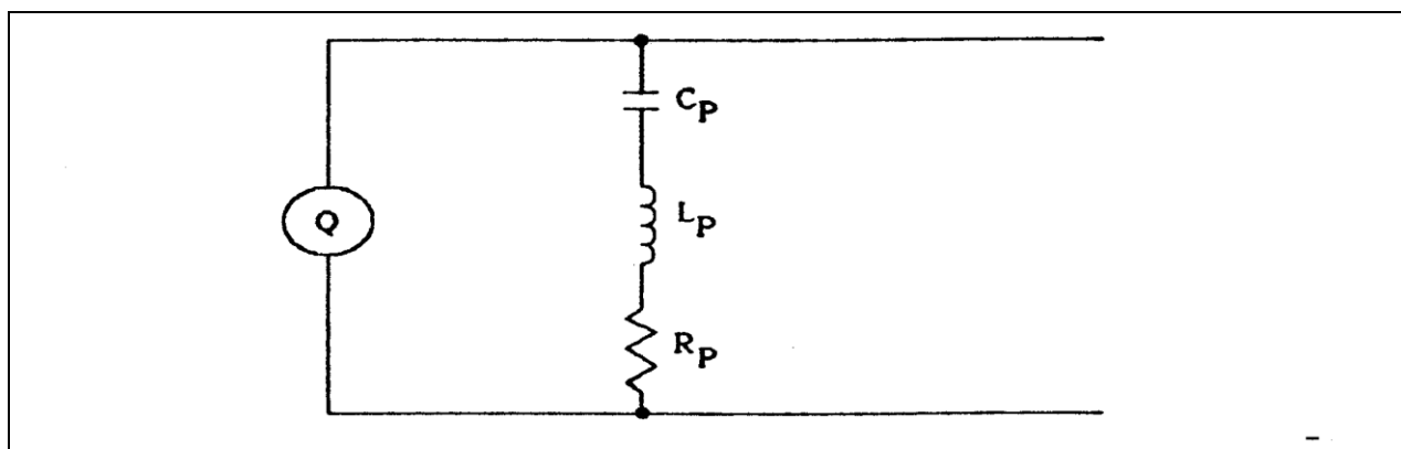
Figure 1-12. Piezoelectric crystal transducer circuit.
