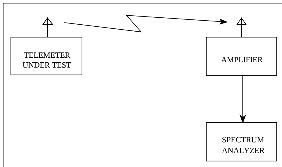
Figure 5-35. Open-air setup.
