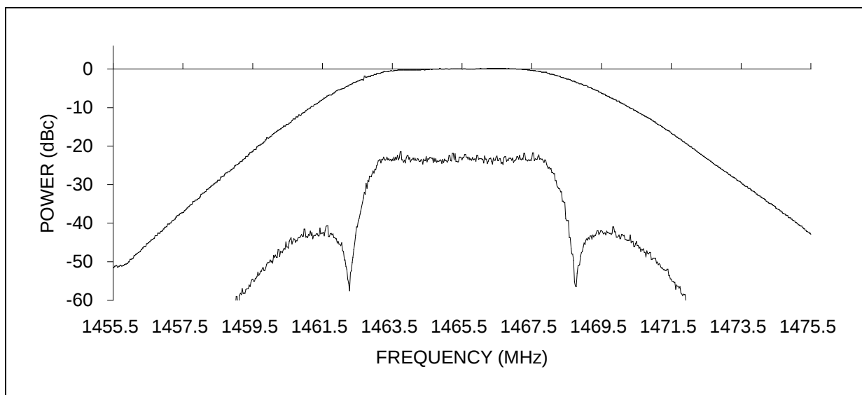
Figure 5-36. Spectrum analyzer calibration of 0 dBc level (modulated carrier).
