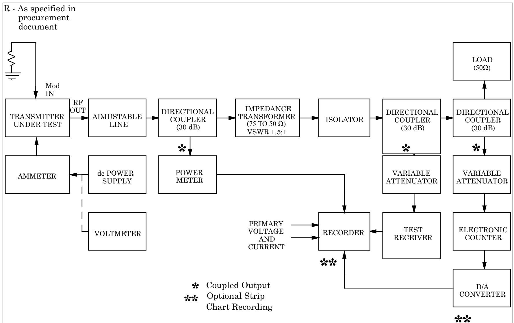
Figure 5-14. Primary power voltage variation test.
