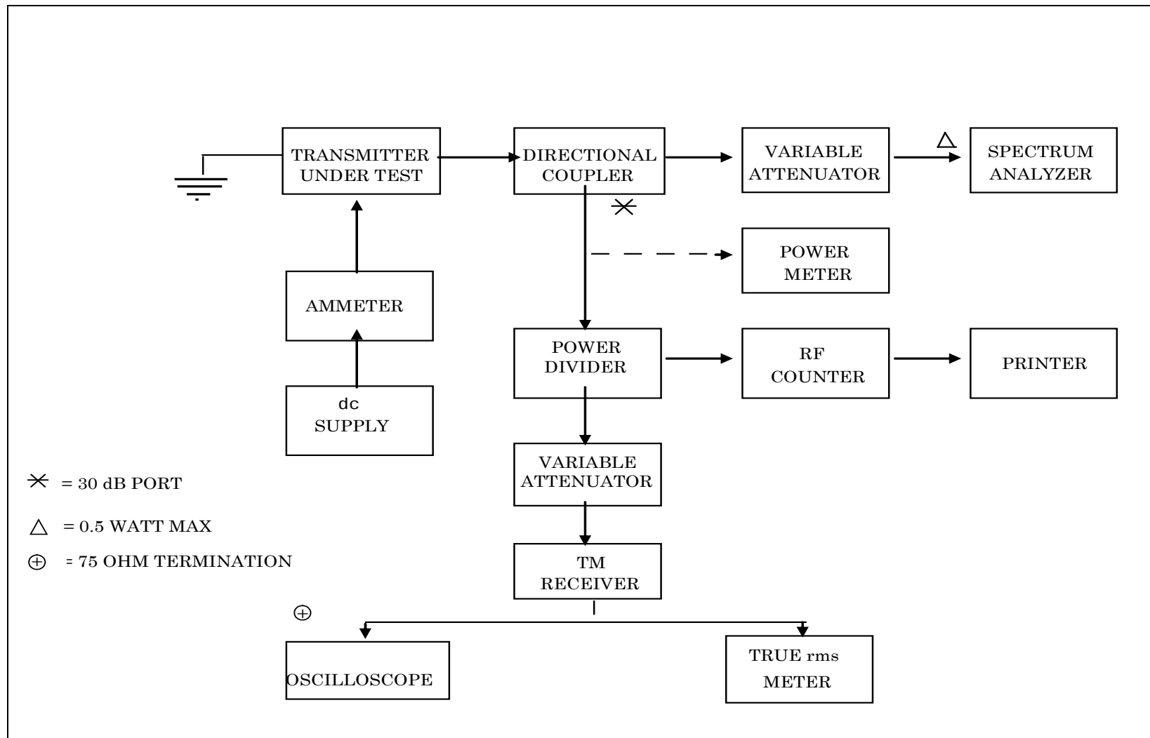
Figure 5-25. Center frequency and frequency stability test setup.
