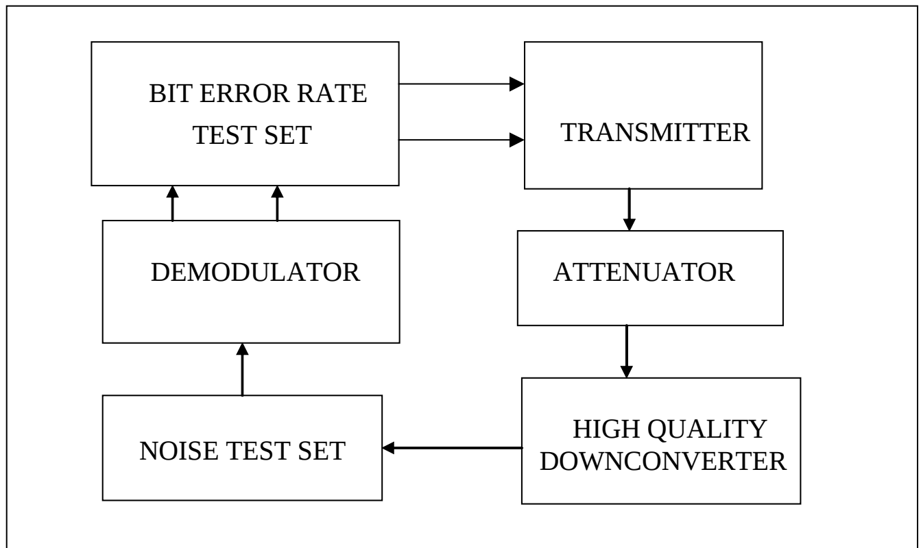
Figure 5-39. Test setup for transmitter bit error probability test.
