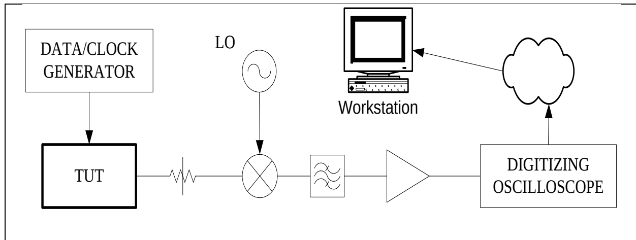
Figure 5-40. Test setup for data digitization and software receiver data processing.
