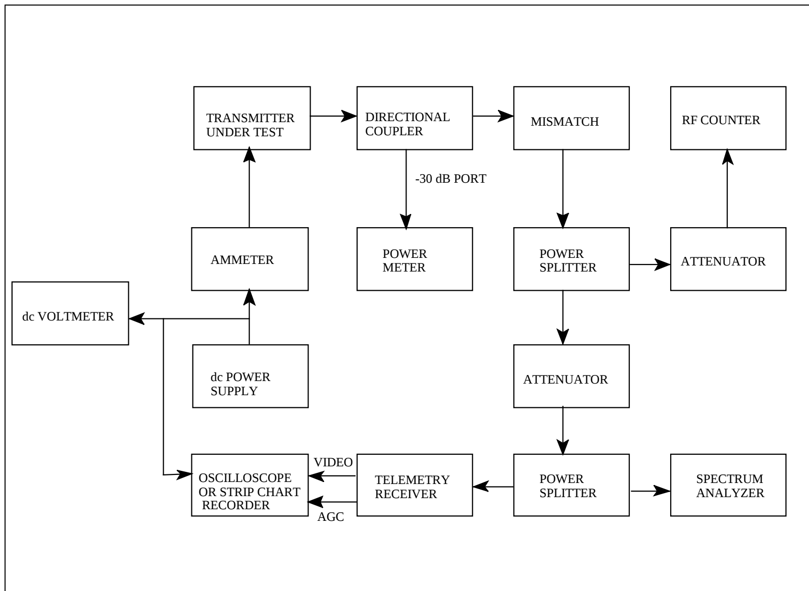
Figure 5-22. Turn-on and turn-off characteristics test.
