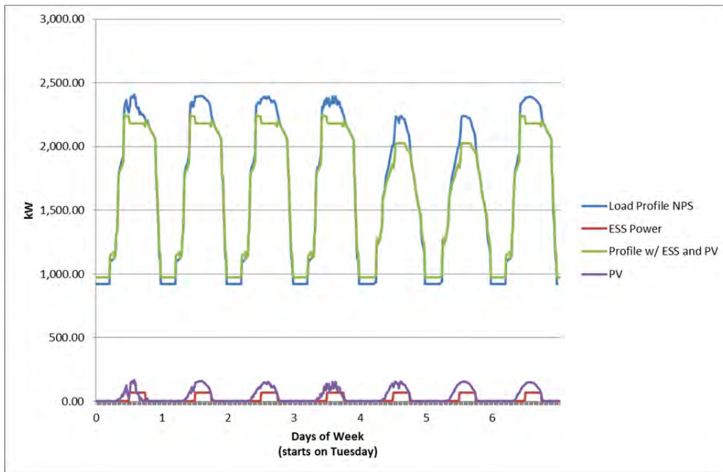
Figure 16. Load profile for the NPS campus with PV and ESS.
