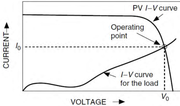
Figure 2. Simplified operating point for load and PV array, from [13].
