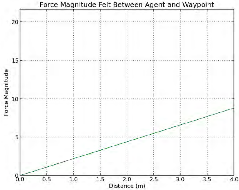
Figure 3.8: This curve describes the force magnitude felt by the agent due to proximity to the current way point ( B = 2.2 ). Unlike the other two force magnitude relationships, force magnitude due to distance from way point is linear.
