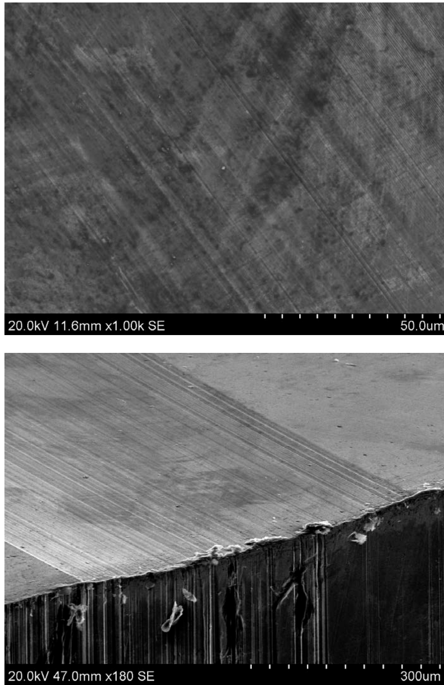
Figure 6-1 - Sample ID: nCoP-1 Wt.% P (AD); SE micrographs of sliding wear track.
