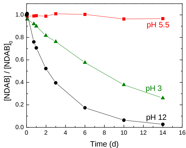
Figure 2.1.3-6. Effect of pH on NDAB degradation in water (150 rpm, 40°C).
