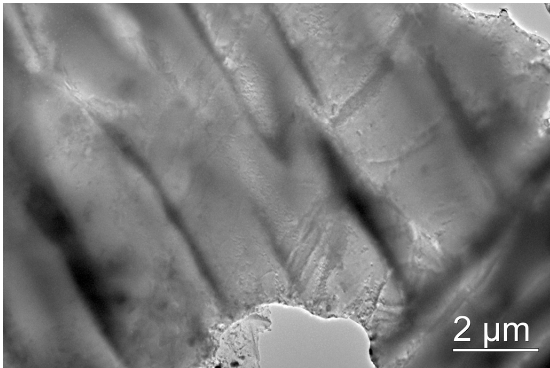
Figure 72. Base metal specimen with defined \alpha and \beta at 940 °C and still contains the \alpha lath structure.
