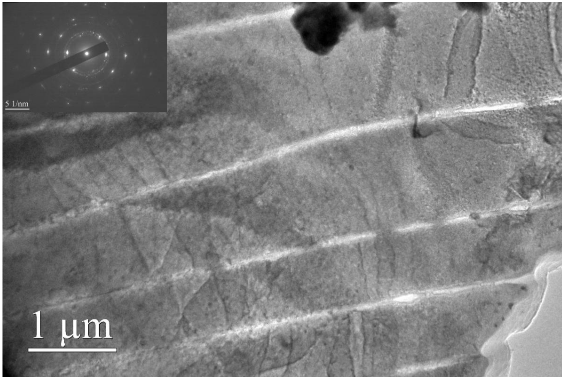
Figure 68. Base metal specimen with defined \alpha and \beta at 949 °C. Rings are noticeable around the diffraction pattern indicating a polycrystalline structure in addition to the large single crystal pattern.
