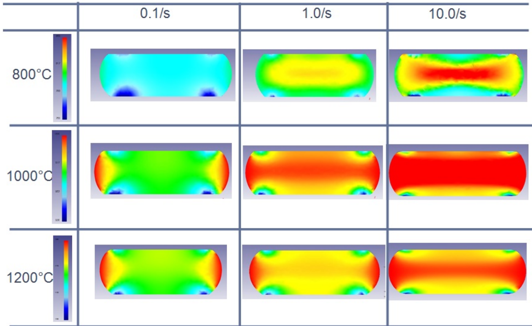
Figure 92. DEFORM compression sections (thermal cross-section) at different strain rates and peak temperatures. As the test temperature decreases from 1200 °C to 800 °C, there is an increased thermal effect due to adiabatic heating during compression.
