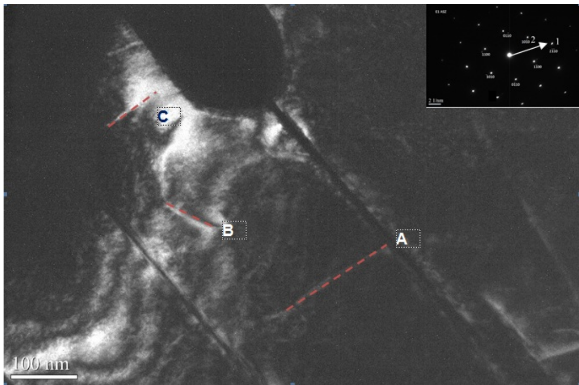
Figure 58. Dark field image from the stir zone for \bar{g} = (2\bar{1}\bar{1}0)
