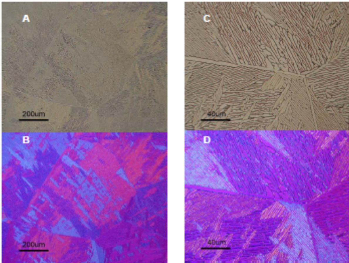
Figure 18. 12.7 mm Base metal optical images. A) 10x magnification of Ti-5111 microstructure consisting of multiple \alpha colonies B) 10x magnification under polarized light C) 50x magnification showing the fully lamellar grain structure D) 50x magnification under polarized light
