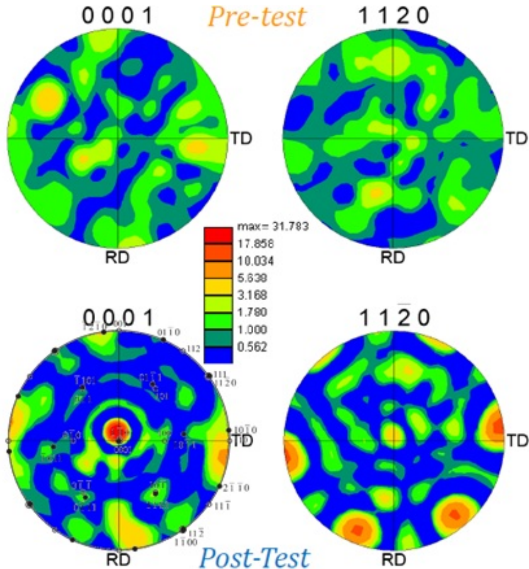
Figure 51. Pre and post microtensile testing texture analysis of all stir zone interface with base metal in Ti-5111. Post-testing shows strengthening in the basal plane texture.
