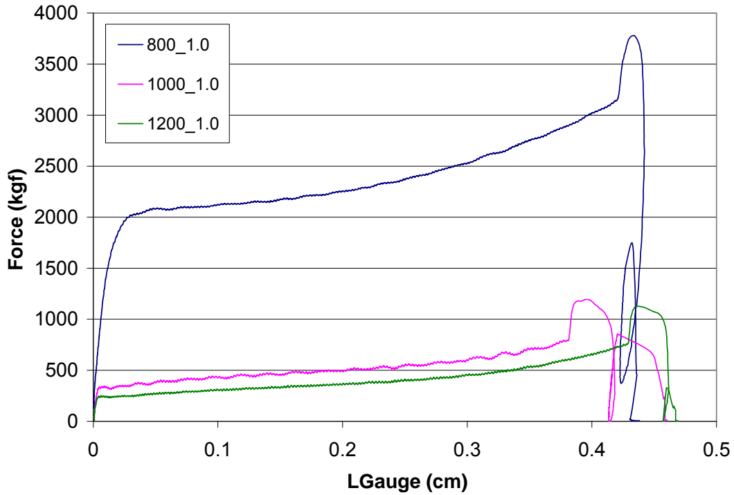
Figure 106. Force curves for water quenched specimens at a constant strain rate of 1.0/s and peak temperatures of 800, 1000, and 1200 C. There is increased force for compression at 800 C.
