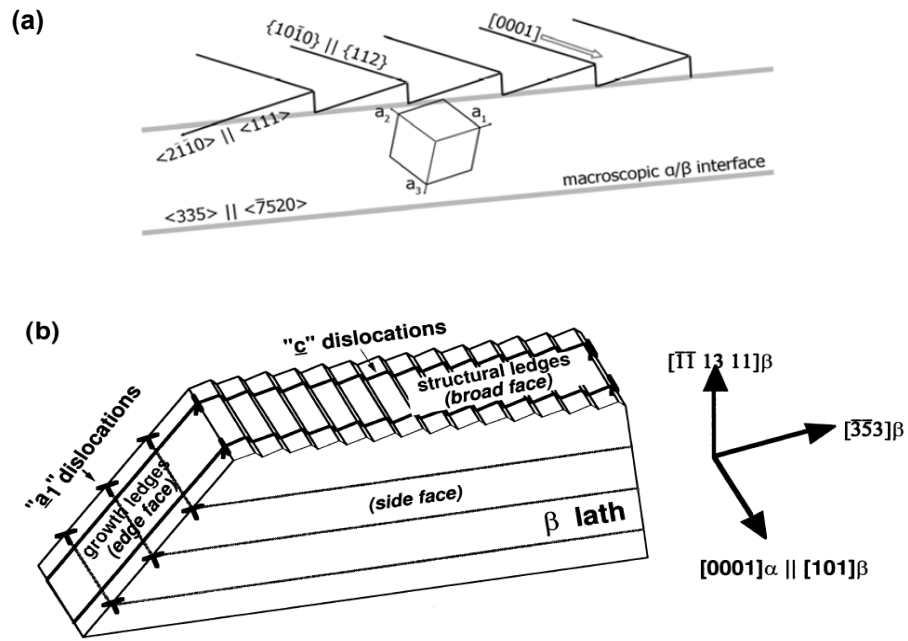
Figure 62. a) Schematic of the \alpha and \beta phase interface. [Pilchak 2009] b) interface structure describing ledges and side face [Suri].
