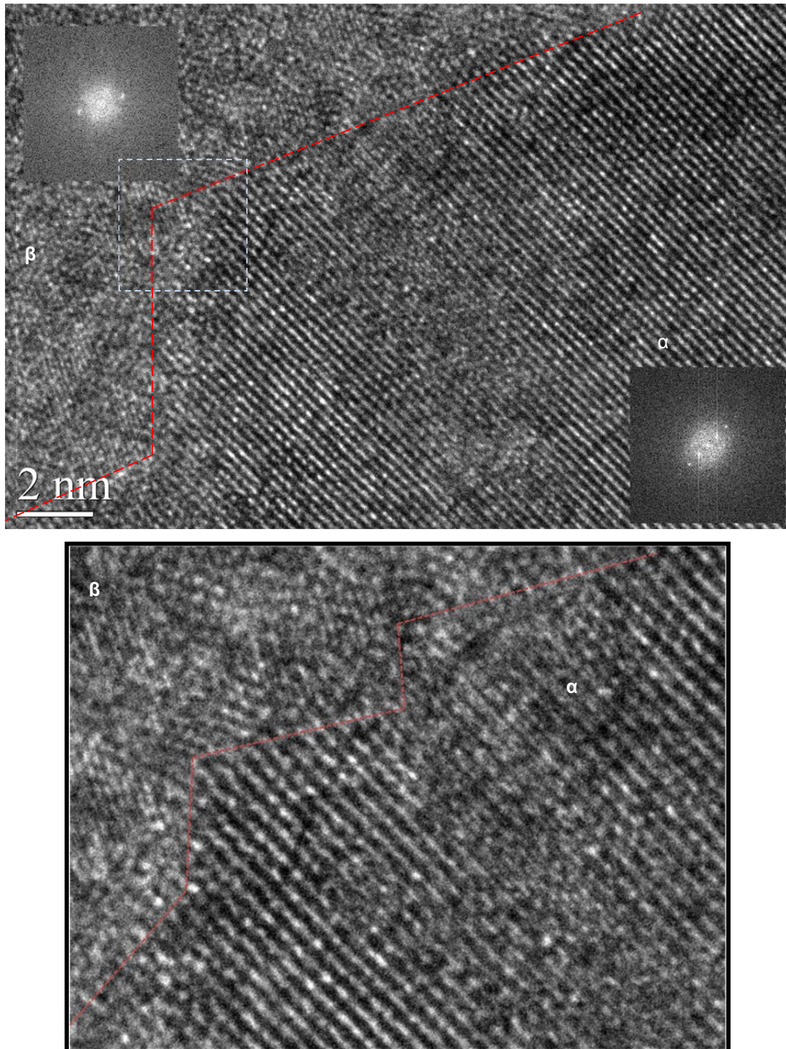
Figure 64. A) High resolution TEM of the \alpha and \beta interface in the base material B) Magnified step of blue box in A. This image shows the atomic level ledges between \alpha and \beta atoms marked by the red dashed line.
