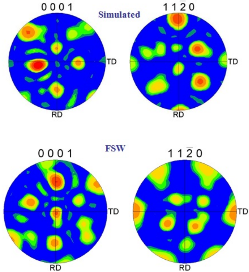
Figure 116. Pole figures of Gleeble FSW thermomechanical simulation at peak temperatures of 1000 °C and a strain rate of 10/s and of the actual FSW stir zone. There is drastic difference in the stereographic projections for (0001) and the (11 \bar{2} 0).
