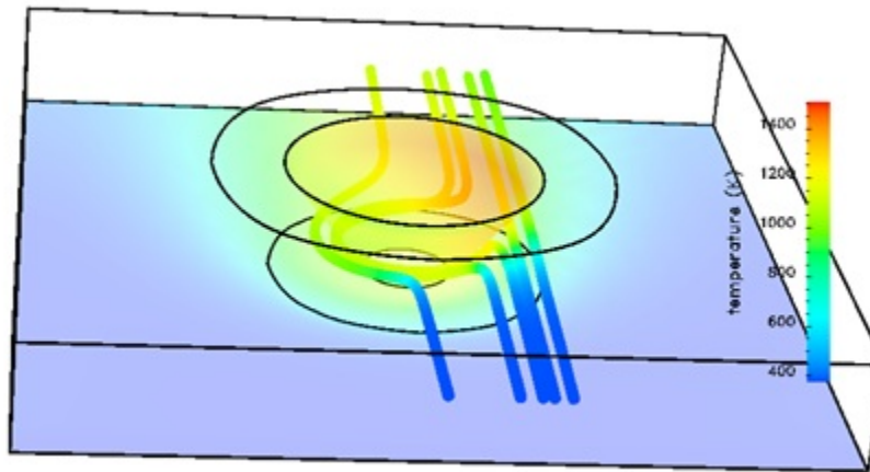
Figure 121. Temperature streamlines with respect to the tool for 12.7mm FSW of Ti-5111 utilizing ISAIH code advancements [Dawson 2010]
