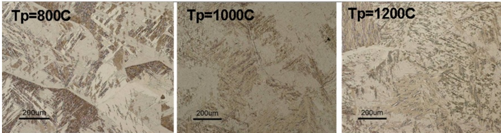
Figure 90. Optical images of simulated specimens with different peak temperatures ( T_p ) and with no deformation
