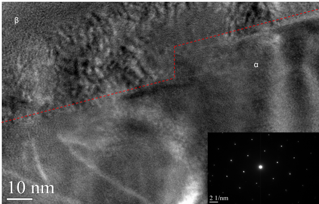
Figure 63. TEM image of the \alpha and \beta interface in base material showing a structural ledge marked with the red line. The selected area diffraction pattern shown in the inset shows that the \alpha lath is oriented along the [0001] direction
