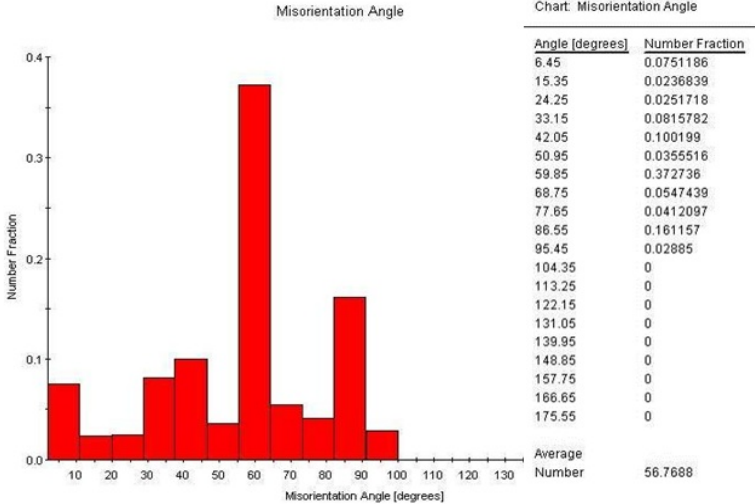
Figure 35. Chart of misorientation angle across the plan view of the weld in Figure 34.
