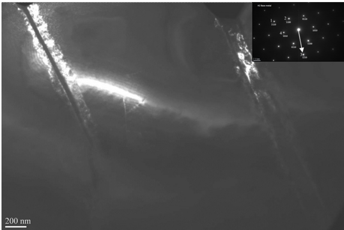
Figure 55. Dark field image from the base metal for \bar{g} = (\bar{1}210)
