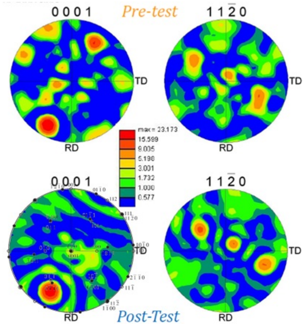
Figure 50. Pre and post microtensile testing texture analysis of all stir zone Ti-5111. Post-testing shows a preference in the BCC and HCP.
