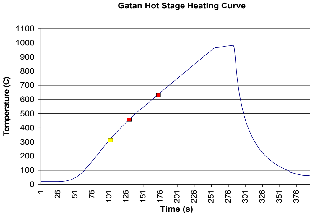
Figure 76. Gatan hot stage heating curve with respect to time for a set heating rate of 1000°C/minute. Yellow box indicates the start of heating. Red boxes indicate points where still video images were taken.
