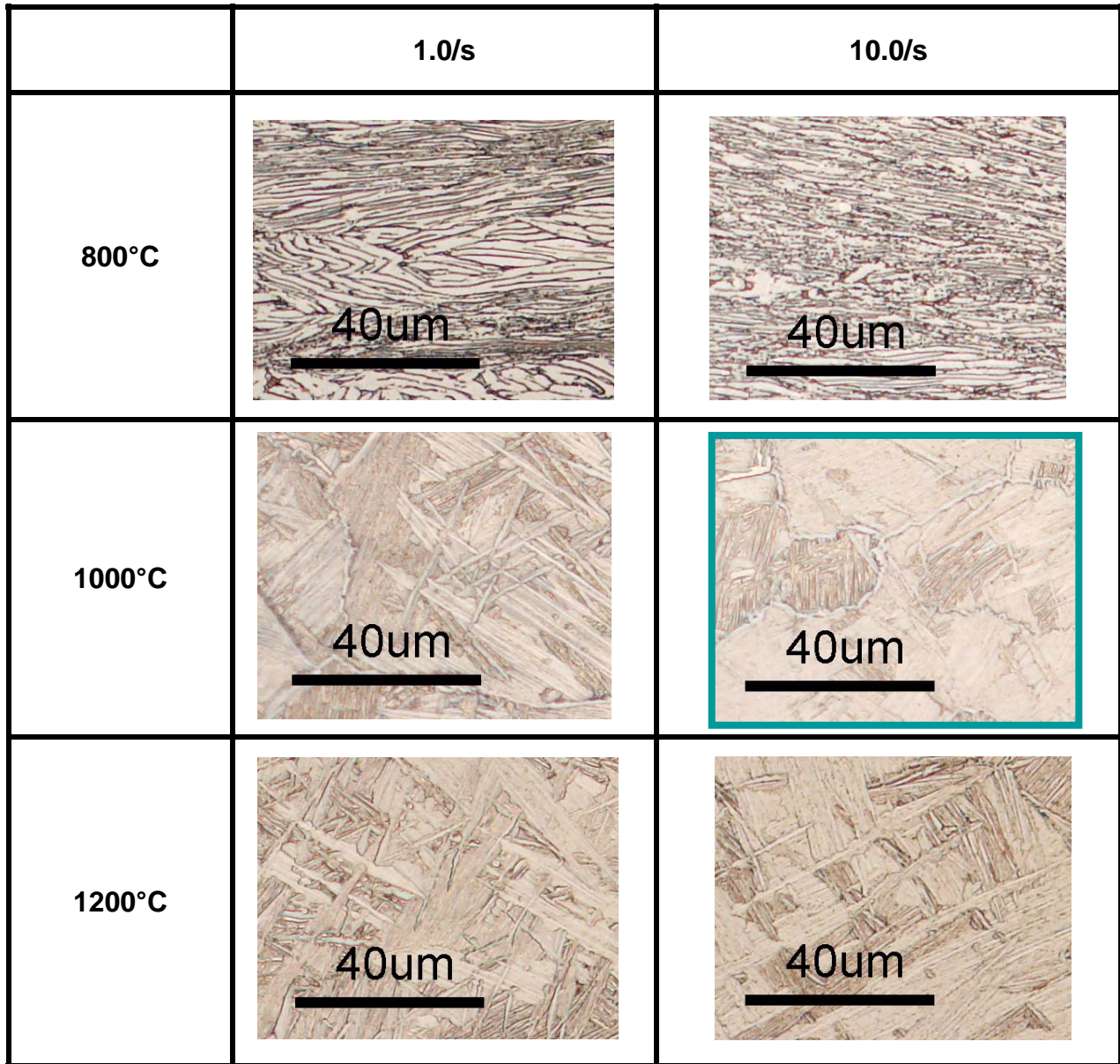
Figure 112. Higher magnification optical micrographs of the center of FSW thermal curve specimens at strain rates of 1.0 and 10.0/s at peak temperatures of 800, 1000, and 1200 C. Subtransus peak temperature (800°C) compression results in \alpha lath bending and kinking (top panel). Dynamic recrystallization for specimens at 1200°C and 1000°C was completed within the \beta phase field resulting in equiaxed microstructure (middle and bottom panel).
