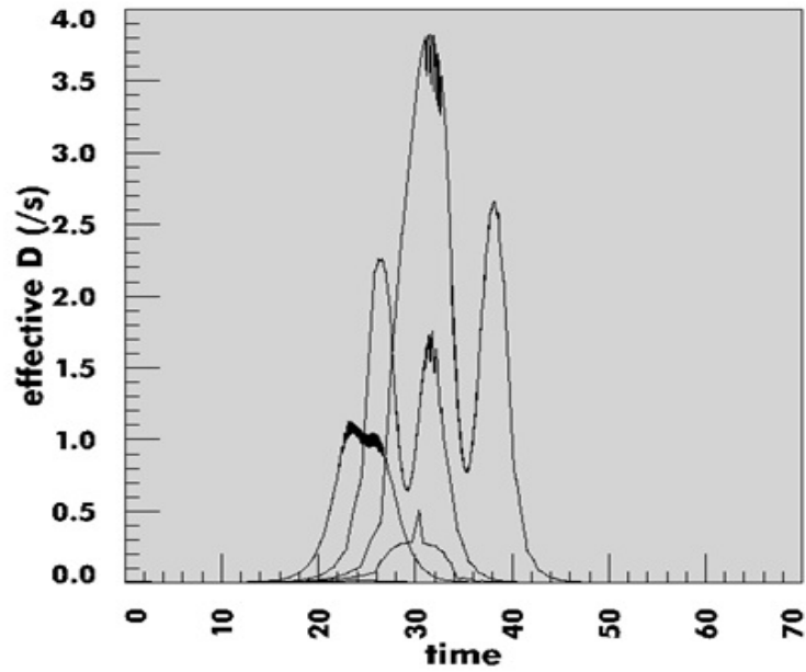
Figure 124. Effective strain rate profile with respect to streamlines in Figure 123 [Dawson 2010]
