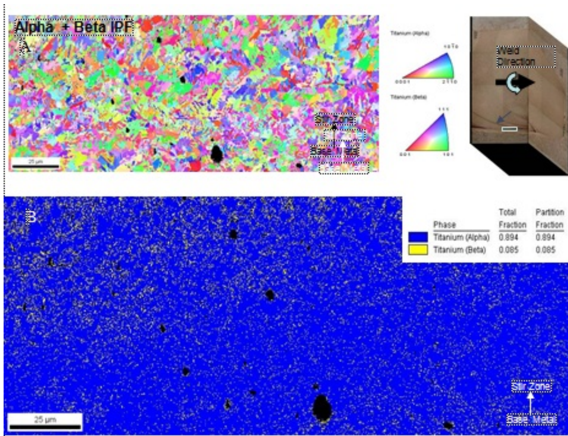
Figure 37. Plan view of 12.7mm Ti-511 FSW. A) Inverse pole figure of the plan view B) Phase map showing \beta -phase surrounding voids shown in black.
