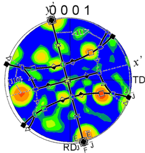
Figure 49. Ideal BCC (110) shear orientation overlaid on the (0001) pole figure from the transition region. Maximum intensity of ODF aligns with strengthening of the F fiber component from BCC simple shear with a rotation of the pole figure by approximately 28.4^\circ about the center of the pole figure.
