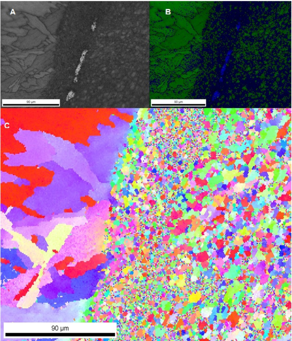
Figure 84. Electron backscatter diffraction of defect marked by the red arrow. (A) Image quality (B) Confidence interval (CI>0.1) (C) Inverse pole figure (IPF)
