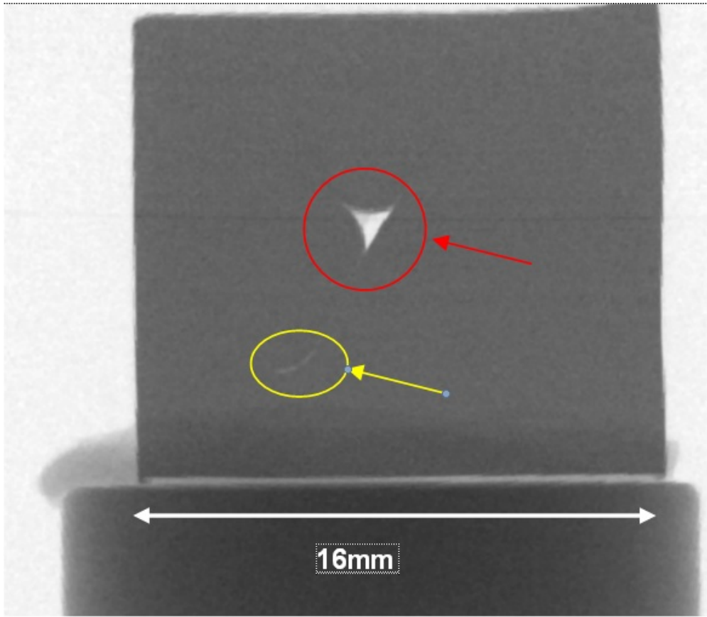
Figure 81. Radiograph (100kV) of a Ti-5111 specimen showing two voided region (arrows) at the interface between the stir zone and the base metal.
