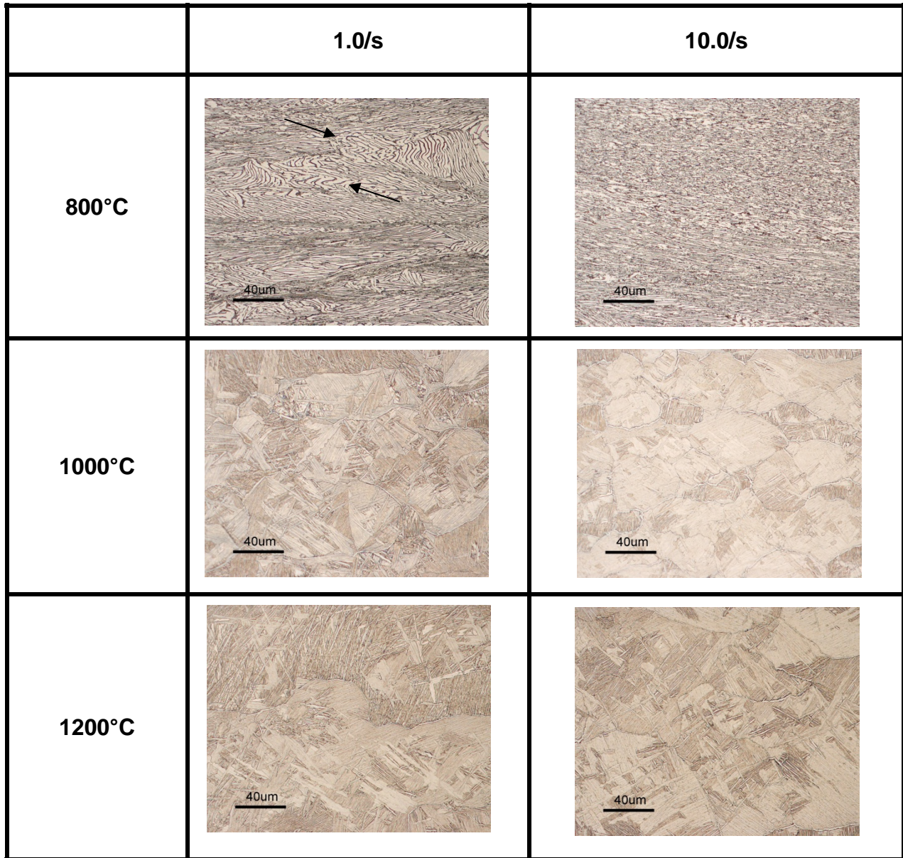
Figure 111. Optical micrographs of the center of compressed specimens using the FSW thermal curve specimens at strain rates of 1.0 and 10.0/s at peak temperatures of 800, 1000, and 1200 C. Arrows show kinking of the \alpha laths below \beta transus (top panel). Dynamic recrystallization for specimens at 1200 °C and 1000 °C was completed within the \beta -phase field resulting in equiaxed microstructure. There is an increased grain size in specimens at 1200 °C due to the longer time spent above \beta -transus.
