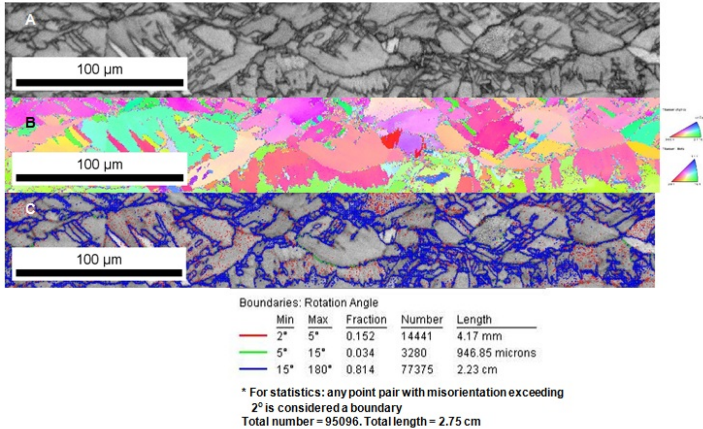
Figure 115. EBSD analysis of Gleeble FSW thermomechanical simulation at peak temperature of 1000 °C and a strain rate of 10/s. A) Image quality map B) Inverse pole figure C) Image quality map overlaid with grain boundary misorientation map
