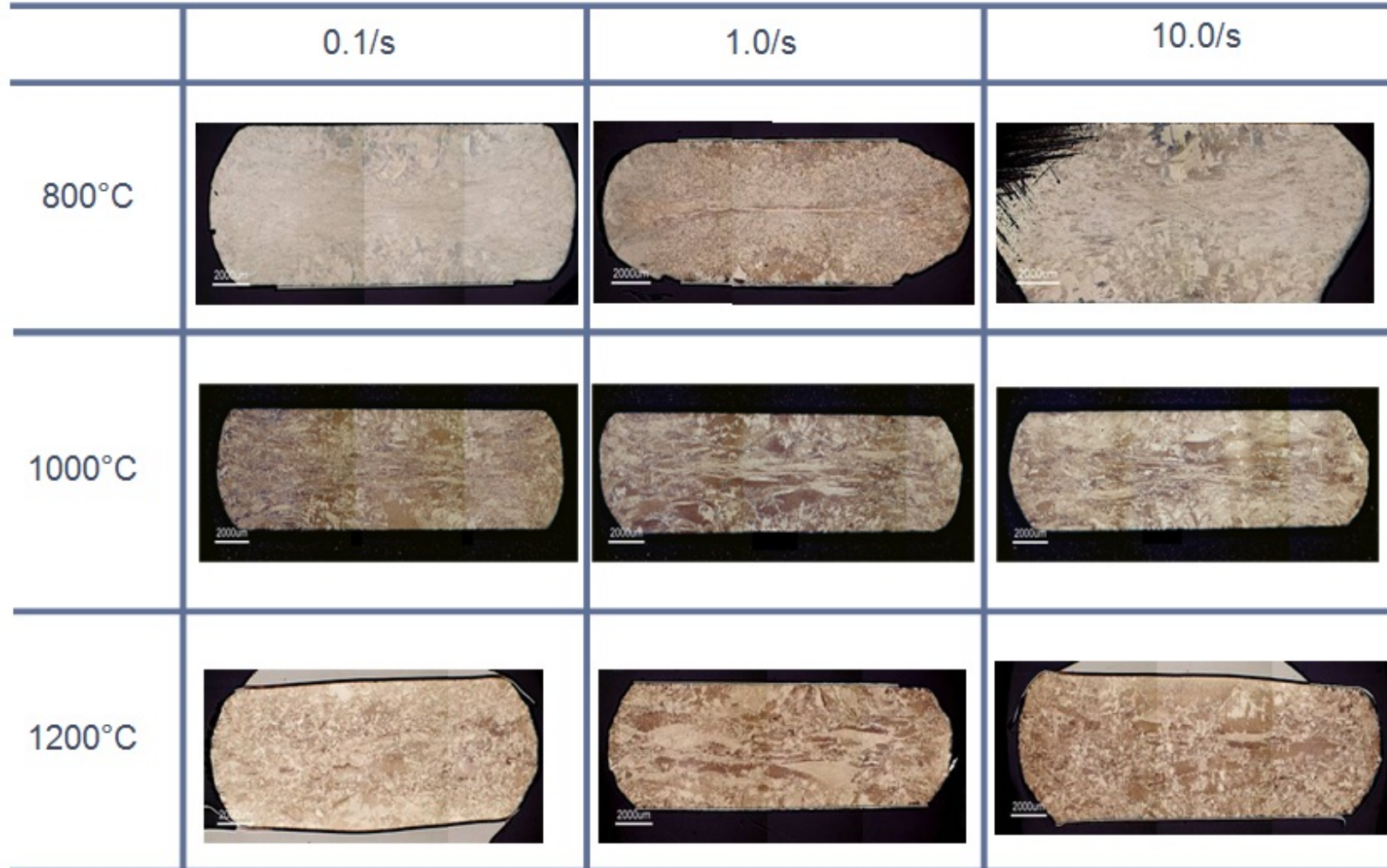
Figure 97. Transverse cross-sections of constant strain rate specimens (0.1, 1.0, 10.0/s) at peak temperatures of 800°C, 1000°C, and 1200°C. There is a difference in compression test barreling below beta transus for different strain rates (top panel). Test specimens at 800°C did not result in full compression at 10/s strain rate. Compression test specimens for 1000°C and 1200°C show even compression through the sample (middle and bottom panel)
