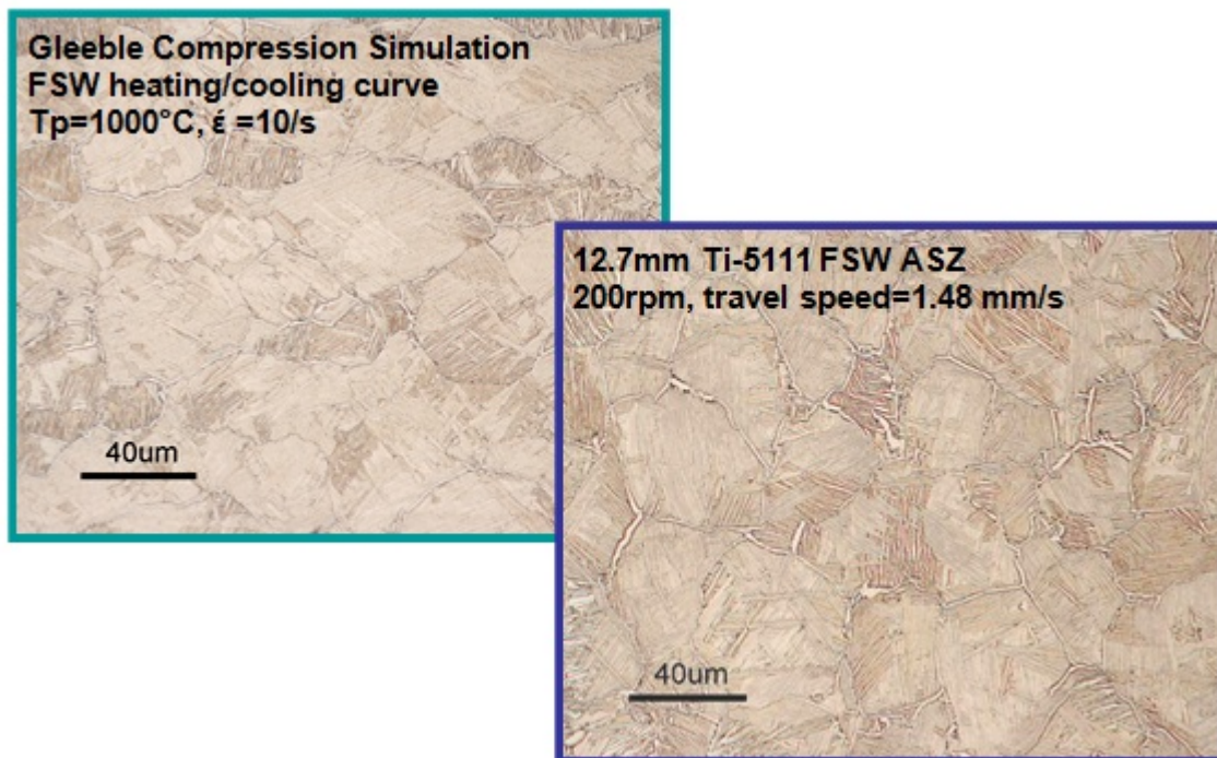
Figure 114. Comparison of the Gleeble FSW thermomechanical simulation at peak temperature of 1000°C and a strain rate of 10/s (left) with the 12.7mm friction stir weld stir zone (right). The two images show similar grain size and \alpha lath width with 2-3 \alpha colonies/grain.
