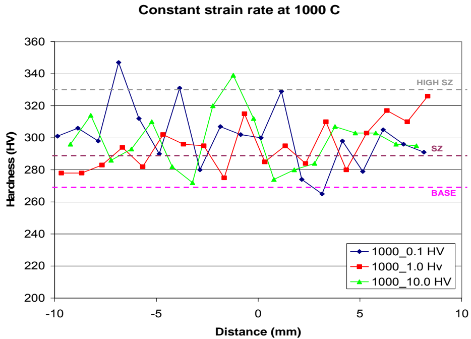
Figure 101. Microhardness traverse along the Gleeble constant strain rate compression specimens at 1000 °C. Hardness values fall in the range for FSW and base metal.
