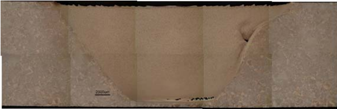
Figure 17. Transverse cross-section of 12.7mm Ti-5111 friction stir weld showing the stir zone, transition region and base metal. Worm-hole defects can be seen at the bottom of the stir zone.
