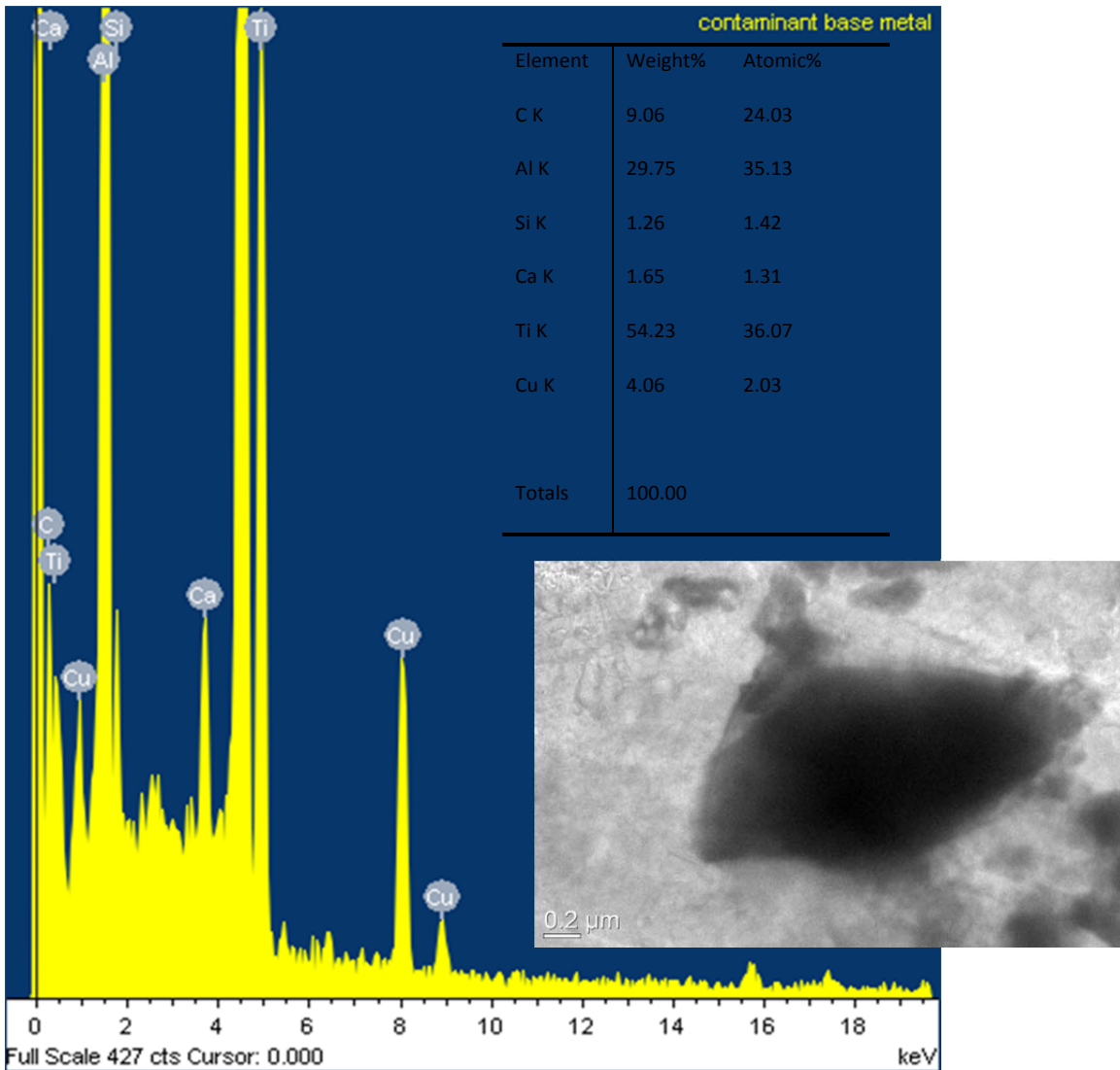
Figure 70. Contamination within the base metal specimen. EDS showing 29.75wt% Al and 4.06wt% Cu. The inset shows a large contaminant in the sample.
