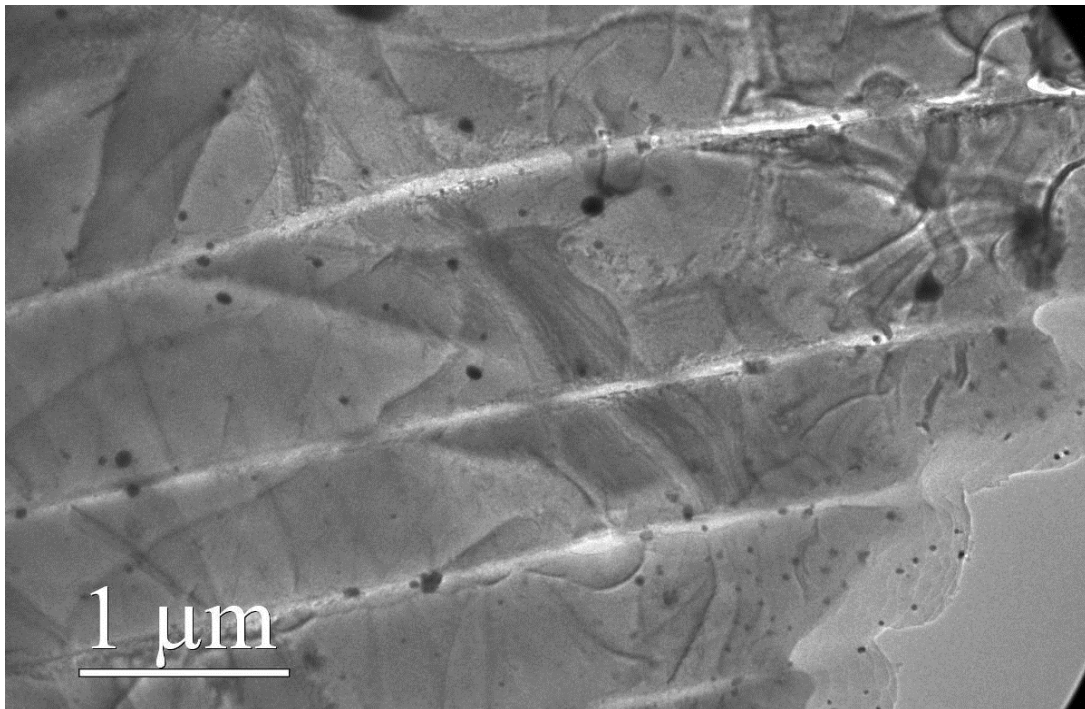
Figure 67. Base metal specimen with defined \alpha and \beta at 640°C.
