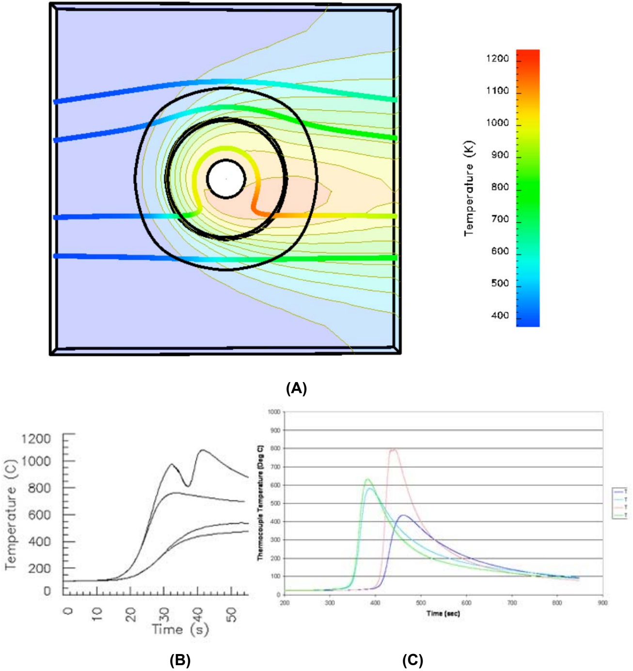
Figure 119. Temperature streamline traces for lower rotational rate of 100rpm A) Streamline with respect to the tool B) Temperature profile with respect to the streamline C) Experimental FSW thermal data at the same respective locations [Dawson 2008]
