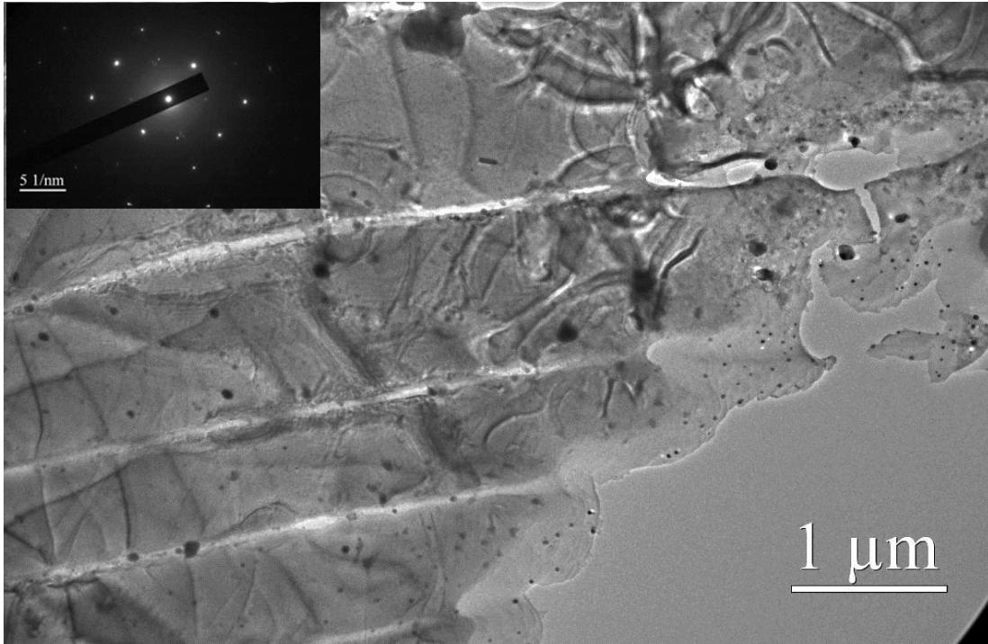
Figure 66. Base metal specimen with defined \alpha and \beta at room temperature and prior to heating.
