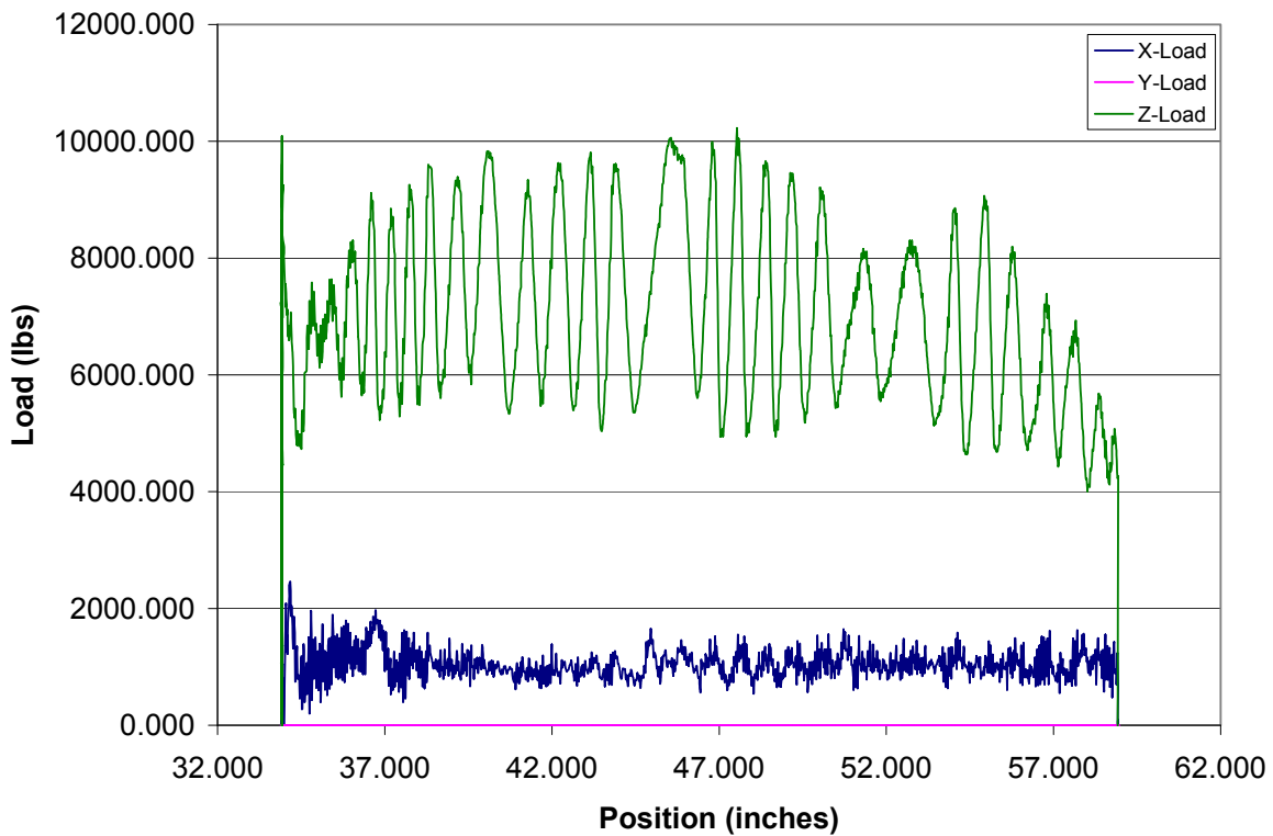
Figure 10. Load data for 12.7mm BJ-12 weld at 1.48mm/s and 200 rpm.
