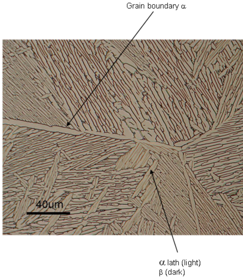
Figure 4. Ti-5111 microstructure (transverse to the rolling direction) showing the typical \alpha+\beta microstructure in Ti-5111.
