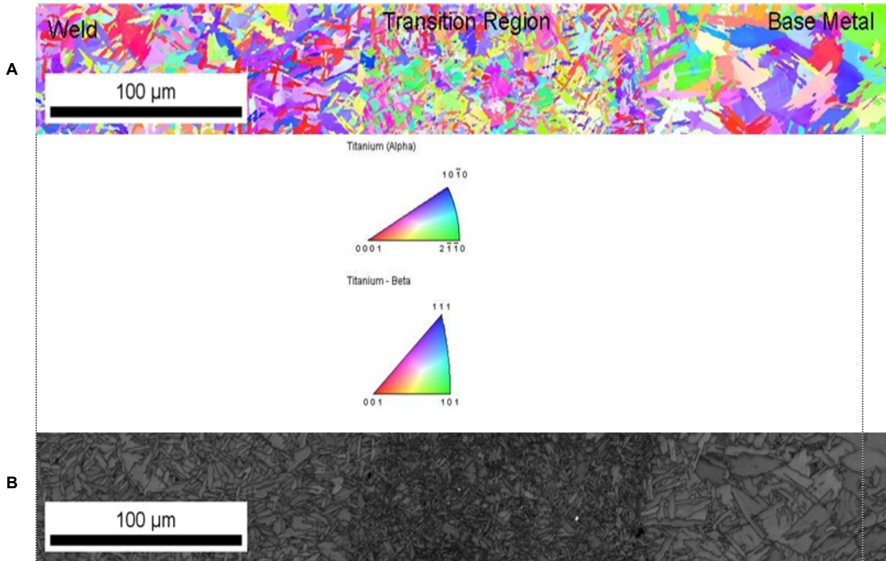
Figure 33. A) Inverse pole figure of the plan view transition region highlighting \alpha colony refinement. The schematic below shows orientations for Ti alpha and Ti beta. B) Image quality map.
