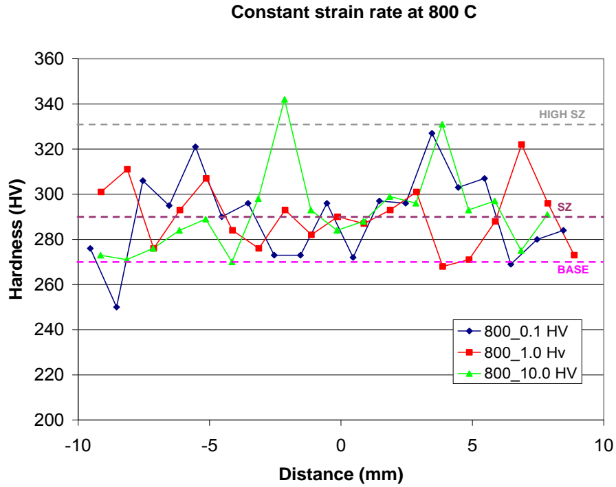
Figure 100. Microhardness traverse along the Gleeble constant strain rate compression specimens at 800 °C. Hardness values fall in the range for FSW and base metal.
