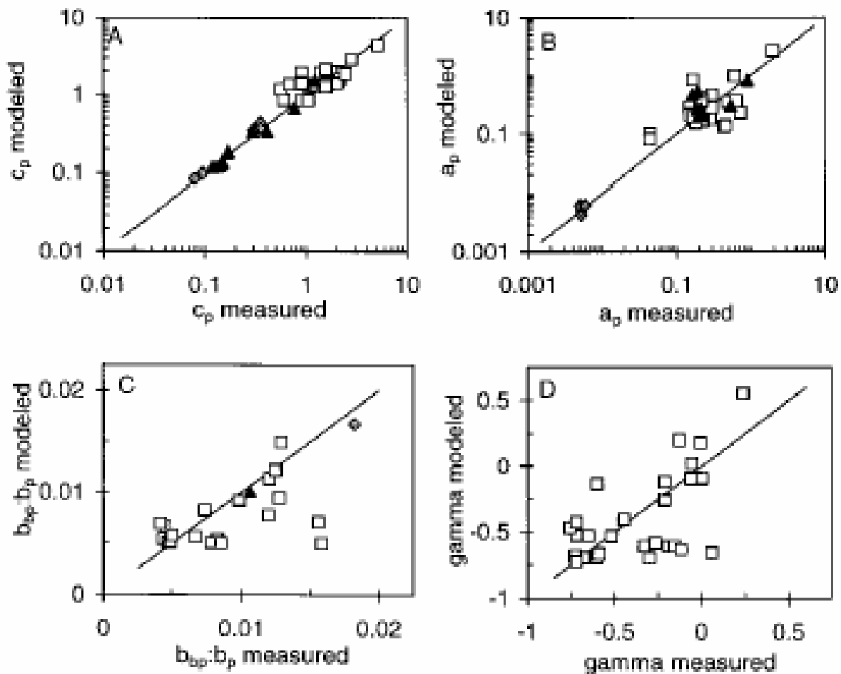
Figure 1. Measured vs. modeled optical properties:[ particulate attenuation (A) and absorption coefficients (B) at 440nm, particulate backscattering ratio at 650nm (C; 532 nm for gyre and Gulf of Maine), and slope of the particulate attenuation spectrum ( \gamma , D). Symbols: gyre - gray diamond, Gulf of Maine - black triangle, Benguela Upwelling - open square.]
