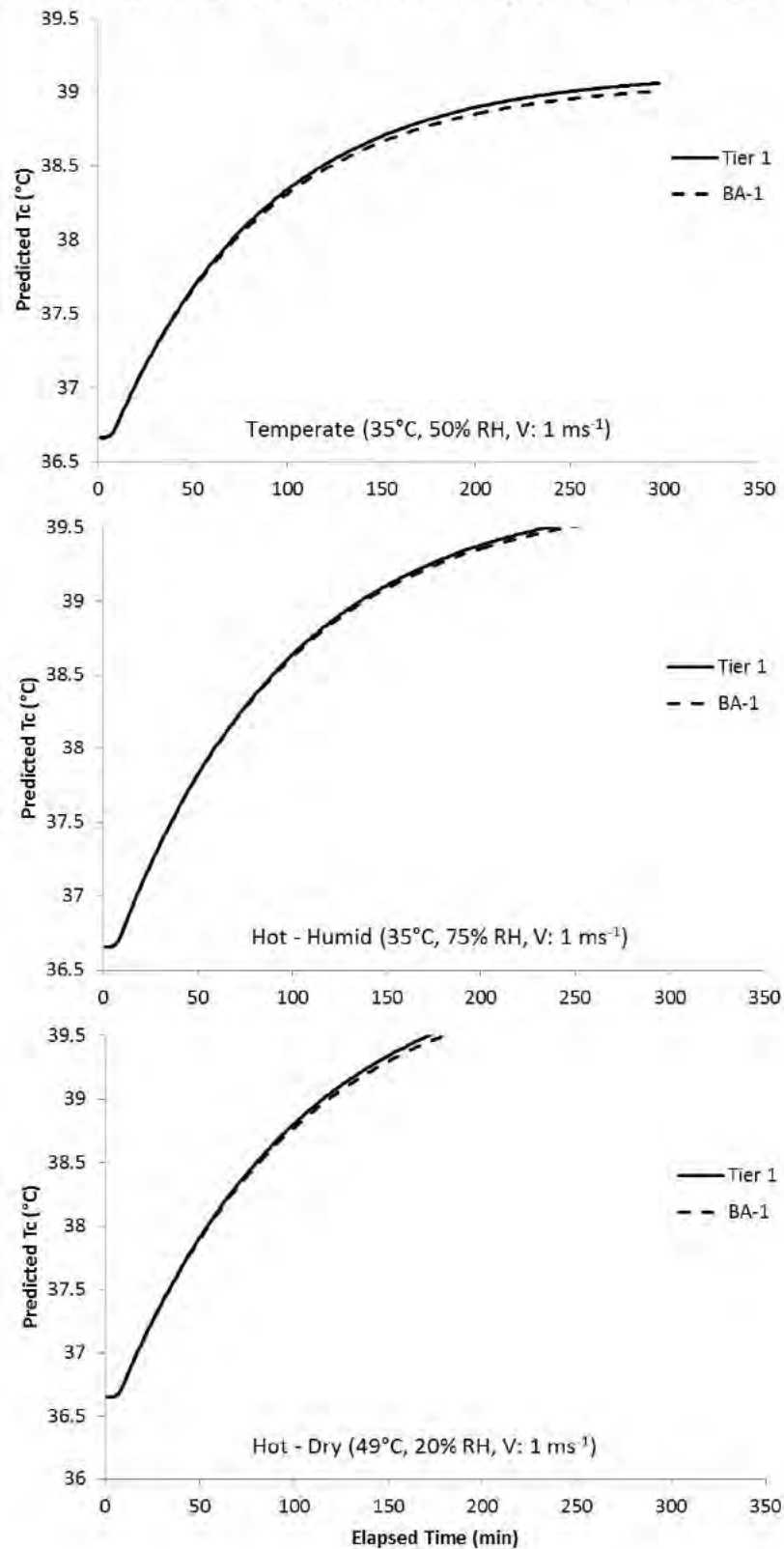
Figure 5. Predicted maximum work times (min) for Tier 1 and BA-1 in no sun, while under temperate, hot-humid (jungle), and hot-dry (desert) conditions
