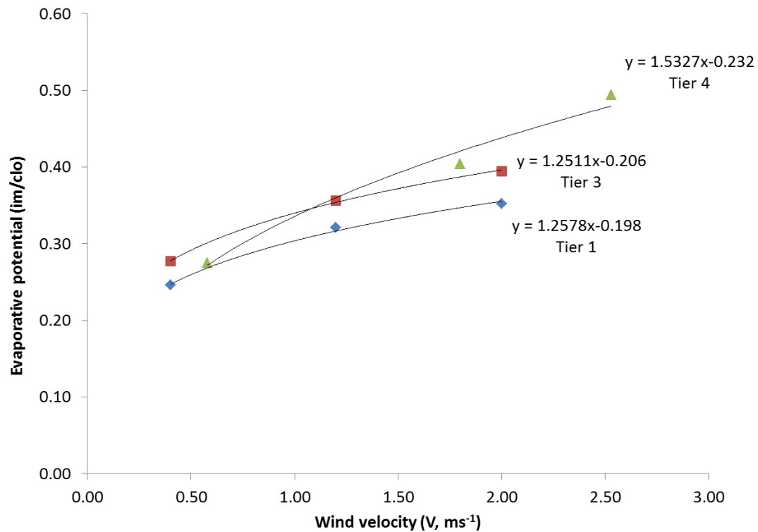
Figure 4. Evaporative potential ( i_m/clo ) for the three prototype body armor (BA) configurations
