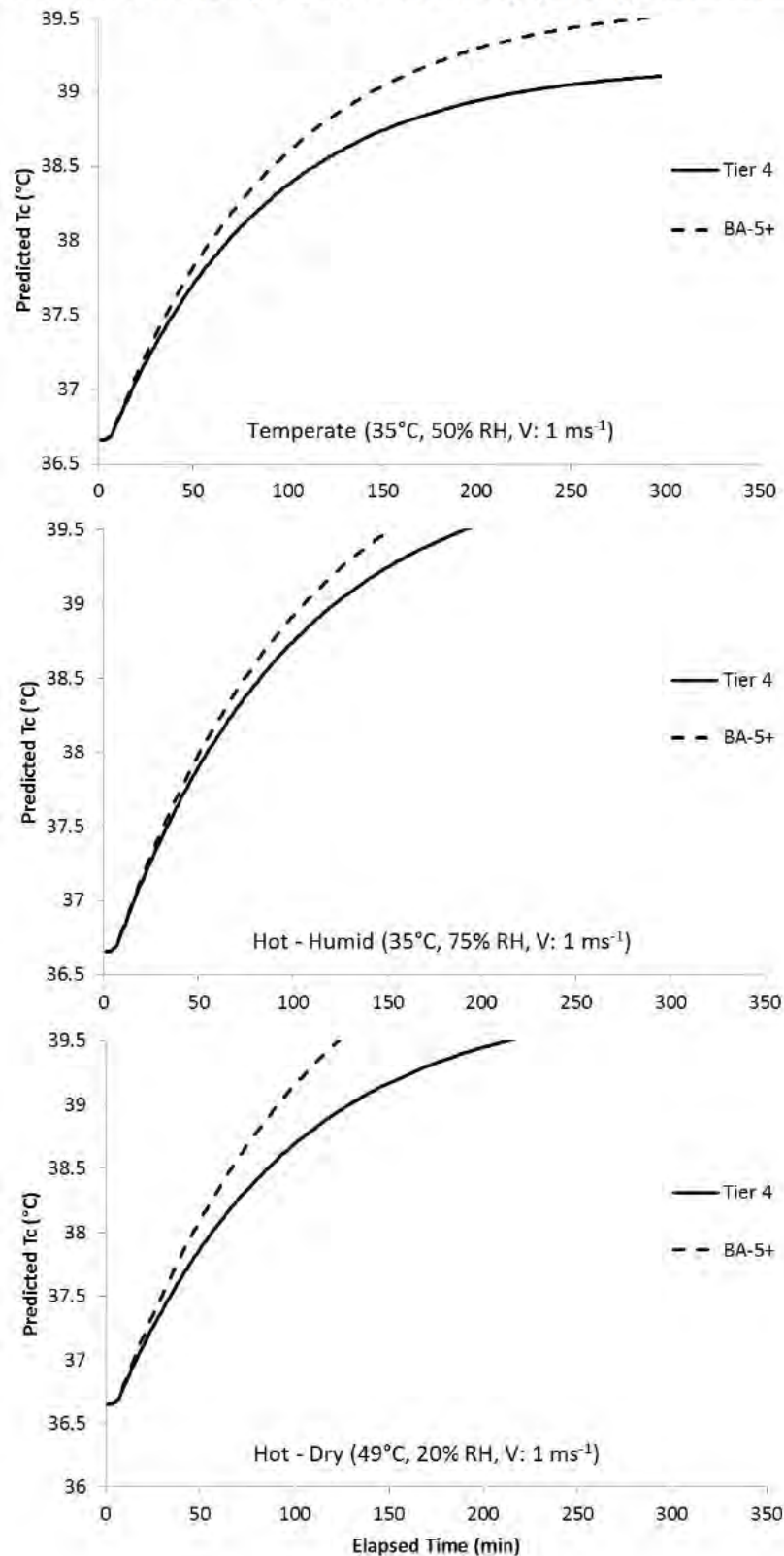
Figure 7. Predicted maximum work times (min) for Tier 4 and BA-5+ in no sun, while under temperate, hot-humid (jungle), and hot-dry (desert) conditions
