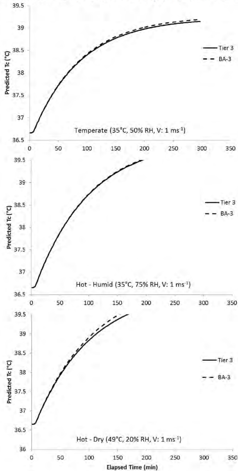
Figure 6. Predicted maximum work times (min) for Tier 3 and BA-3 in no sun, while under temperate, hot-humid (jungle), and hot-dry (desert) conditions
