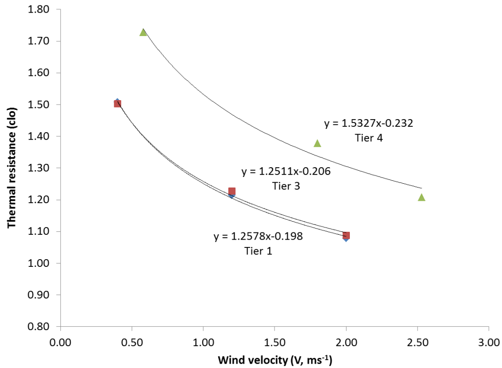
Figure 3. Thermal resistance (clo) for the three prototype body armor (BA) configurations
