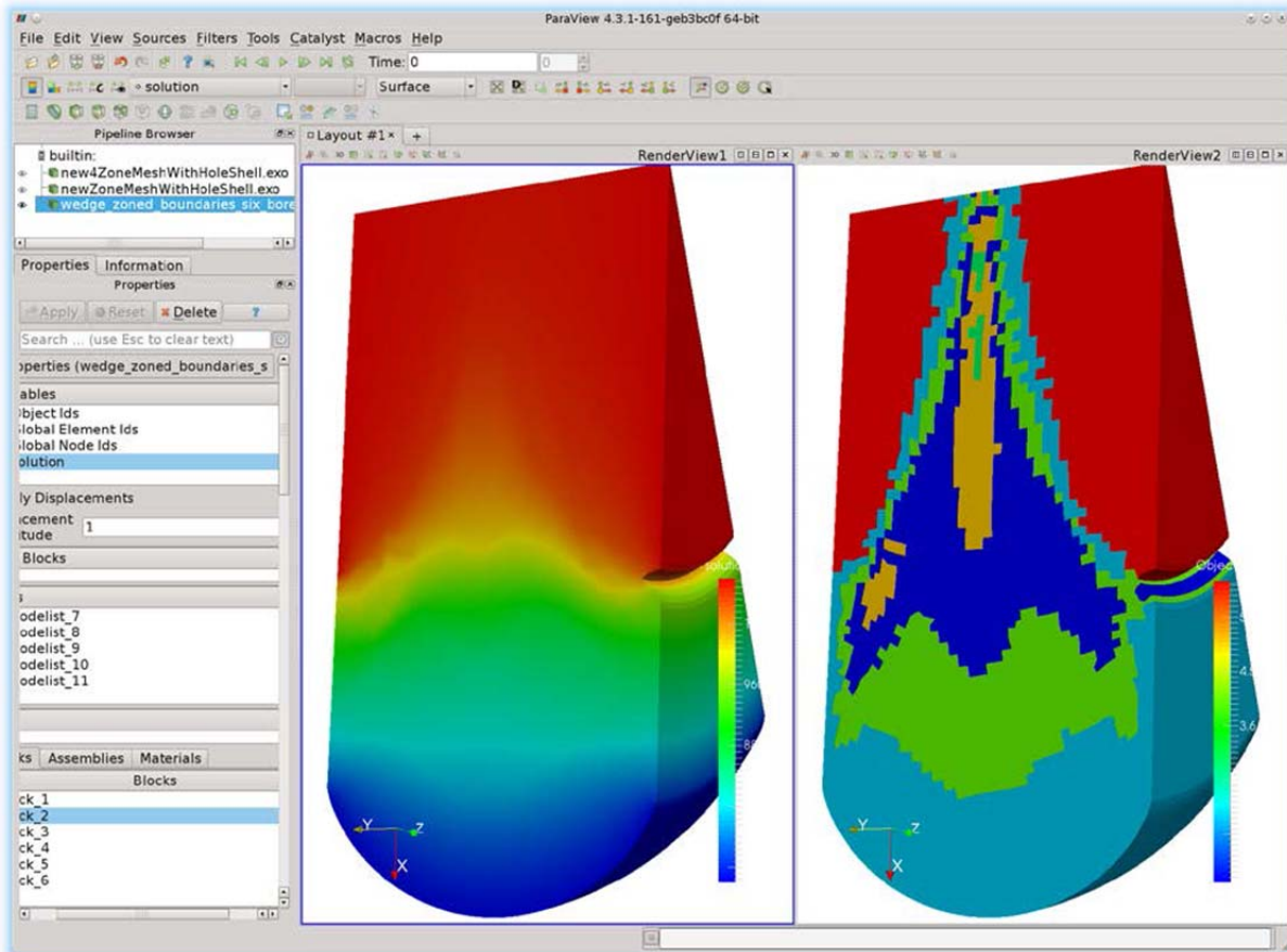
Figure 16. ParaView Showing Analysis of Albany Simulation
