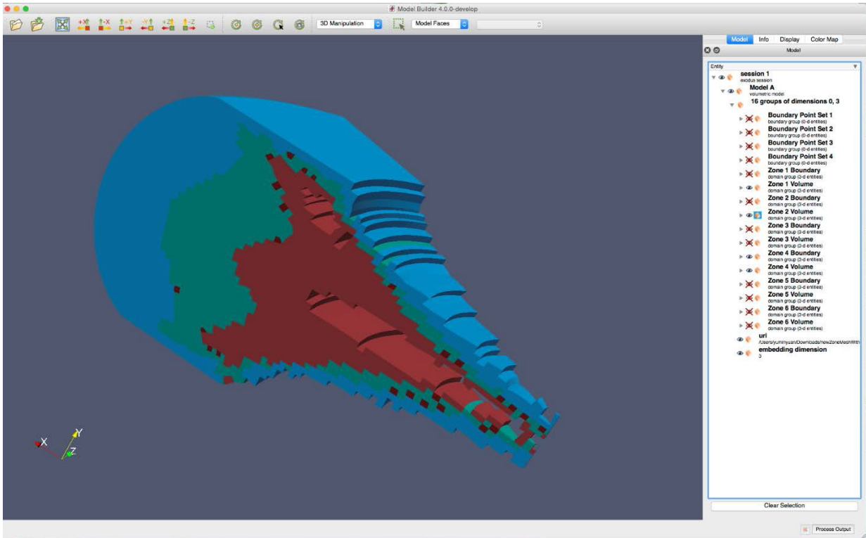
Figure 15. The Zoned Wedge Geometry in Computational Model Builder
