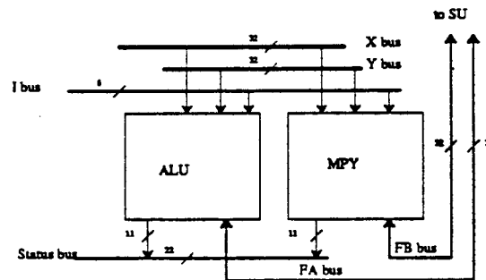
Figure 12: Execution Unit Block Diagram
