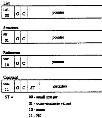
Figure 2: PLM Data Tagging Representation
