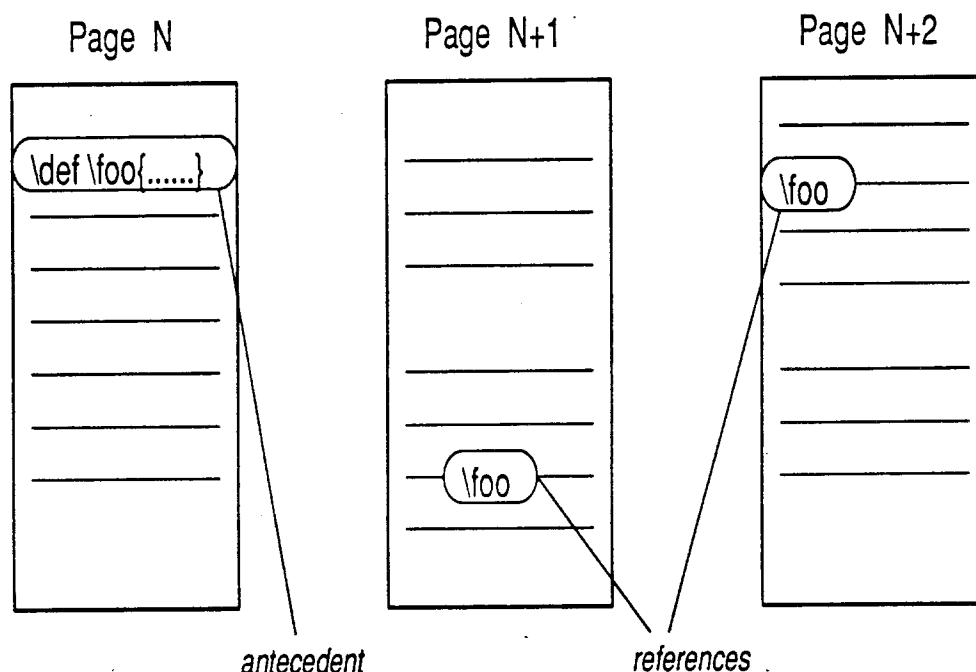
Figure 7.1: Caller/callee name dependence . This example shows the definition of a macro on page N and two separate invocations in the remaining context of the document. When the definition of the macro is changed, the references (invocations) become invalid and consequently their enclosing objects (e.g., pages N + 1 and N + 2 ) must be reprocessed.
