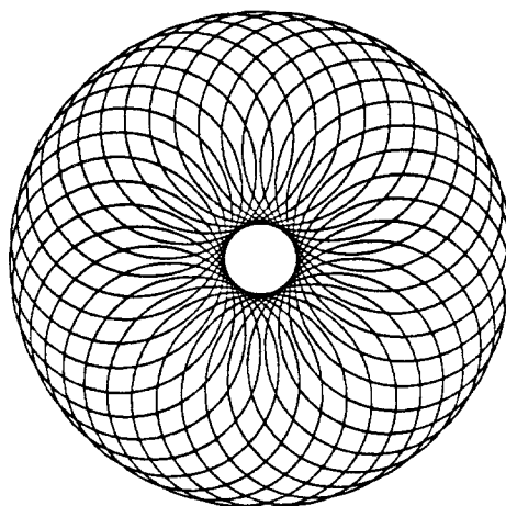
Figure 3.3: Rotated circles . A set of rotated circles and the corresponding PostScript code used to generate it. PostScript has a postfix syntax, so the one line code here means iterate a procedure 36 times. In each iteration first a circle centered at (60, 0) with a radius of 45 is drawn (in points), then the coordinate system is rotated by 10 degrees.
