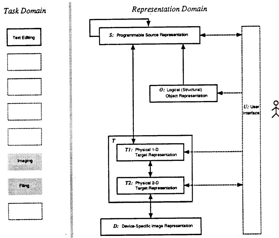
Figure 4.3: Graphical representation instantiation of Emacs . The task of text editing has been singled out by the darkened box on the left. The shaded boxes represent other tasks involved in the overall system that are not the focus of current instantiation. Empty boxes are those tasks that play no roles in the system.
