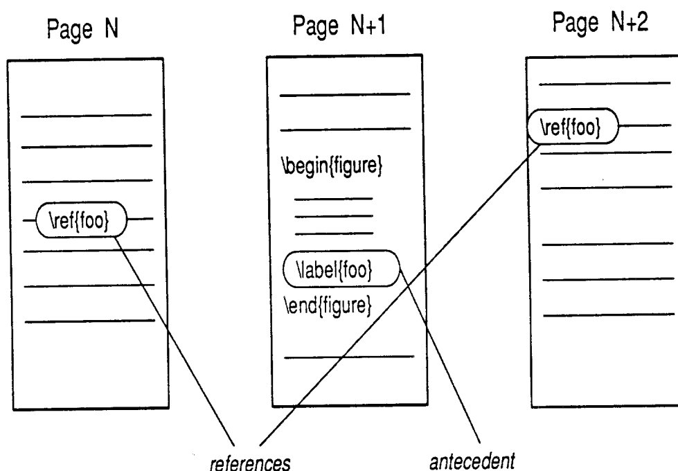
Figure 7.2: Cross-referencing attribute dependence . This is an example of cross referencing in a document. An antecedent is labeled somewhere and references can appear anywhere else. Usually it is not the content of an antecedent like this that matters. What matters is their ordering with respect to similar objects. When an antecedent changes its relative position in the document, multiple passes are needed to bring the references up to date.
