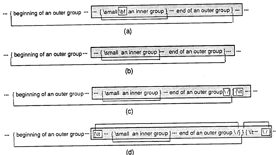
Figure 6.9: Full treatment of region font change (case 1) . The figure shows the stepwise development of region font change. The shaded area denotes the region, in which unshaded areas are text to be deleted or just inserted. Lines connecting matching opening and closing delimiters of a group illustrates its scope. (a) An outer group's right branch overlaps with the region; an inner group inside the region contains a font invocation ( \bf ). (b) After font-remove , \bf is stripped off. (c) Extra delimiters are inserted by group-rearrange . (d) Finally, following font-change , the new font \it is embedded in the region under two separate groups.
