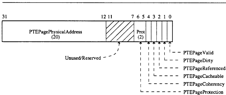
Figure 2.4: Pagetable Entry (PTE) Format
