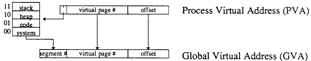
Figure 2.2: Formation of Global Virtual Address
