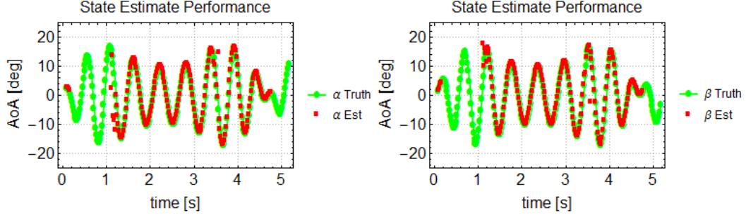
Fig. 6 Estimate of pitch and yaw angles of attack using perfect OF
