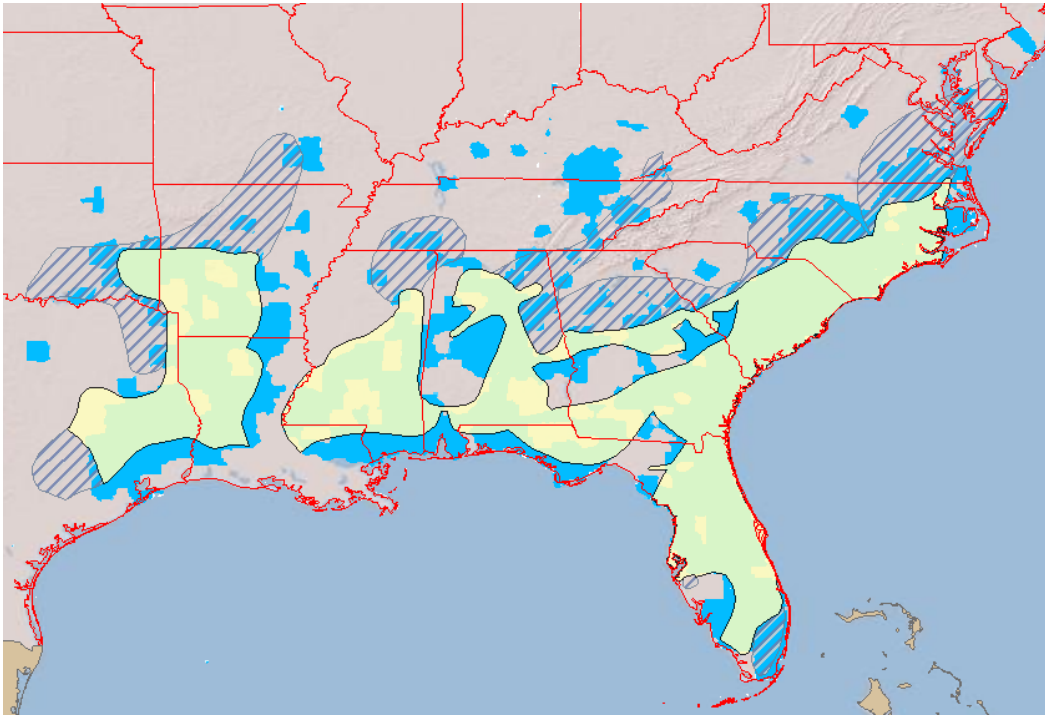
Figure 1. Plots of contradictory RCW range data.
