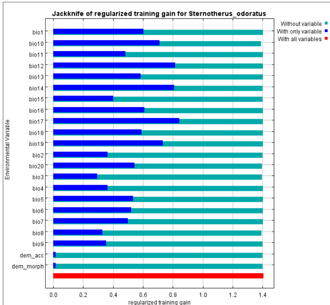
Figure 32. Jackknife analysis for the gains in viability based on the “training” locations.
