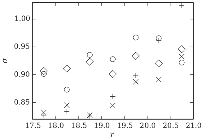
Figure 9. Standard deviation of the distribution of QSO proper motions divided by proper motion errors, in half-magnitude bins. Circles and diamonds are the standard deviations in R.A. and decl., respectively, for the Bok survey. Pluses and crosses are the standard deviations in R.A. and decl., respectively, for the 1.3 m survey. Perfectly estimated errors would yield a standard deviation of one.
