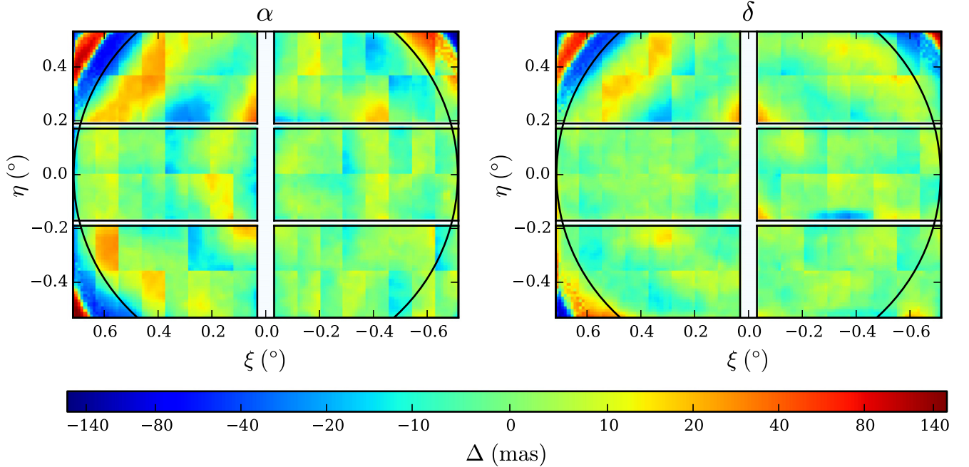
Figure 4. Map showing the mean residuals (catalog–observed, in mas) across the focal plane for the 1.3 m survey. Residuals in R.A. are shown in the left panel, and in decl. in the right panel. A circle with radius 0.7^\circ is shown for reference.
