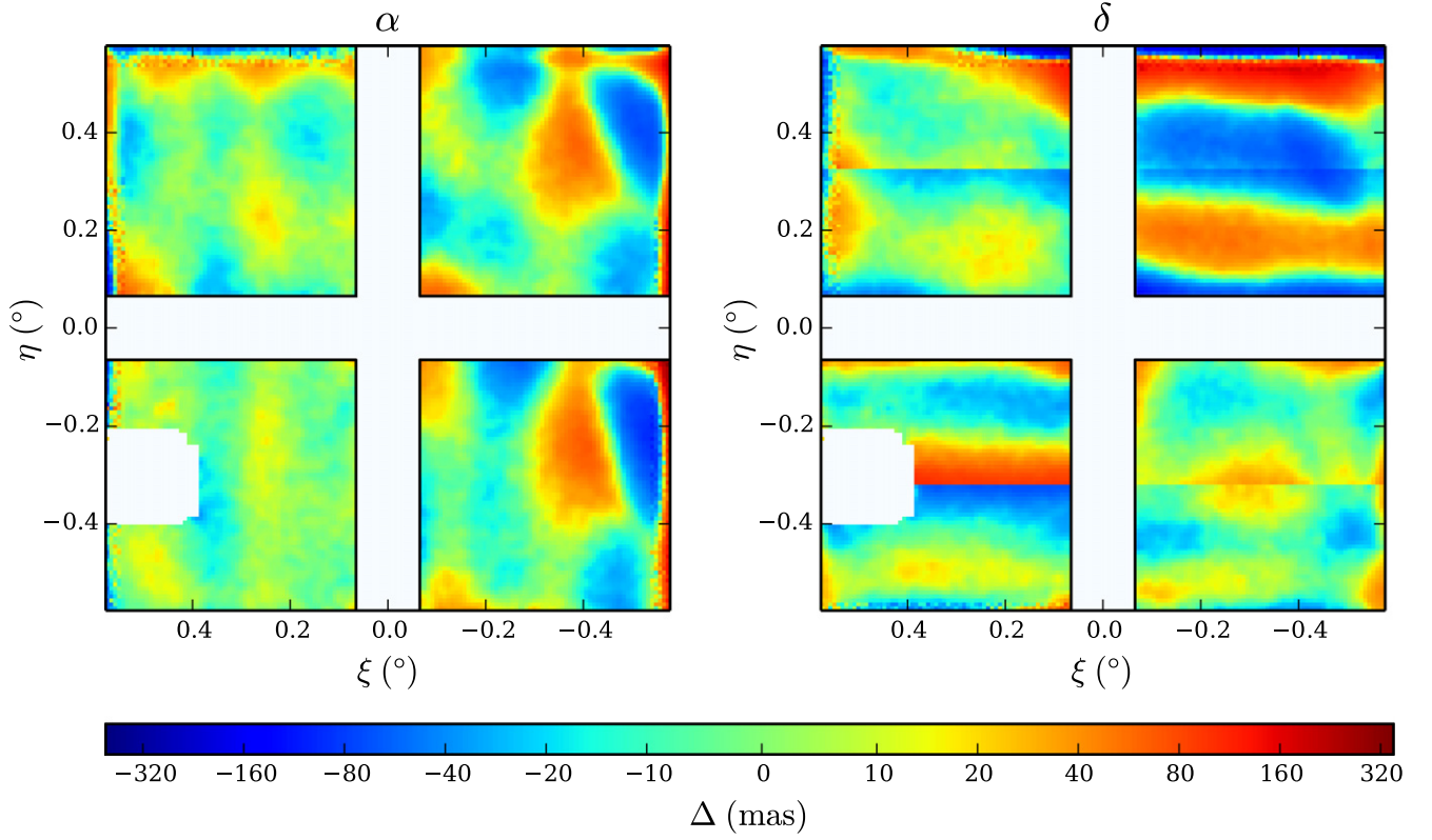
Figure 3. Map showing the mean residuals (catalog–observed, in mas) across the focal plane for the 2008 Bok runs. Residuals in R.A. are shown in the left panel, and in decl. in the right panel.
