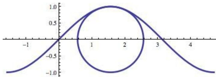
Figure 6.1. The geometric basis for the calculation of curvature.
