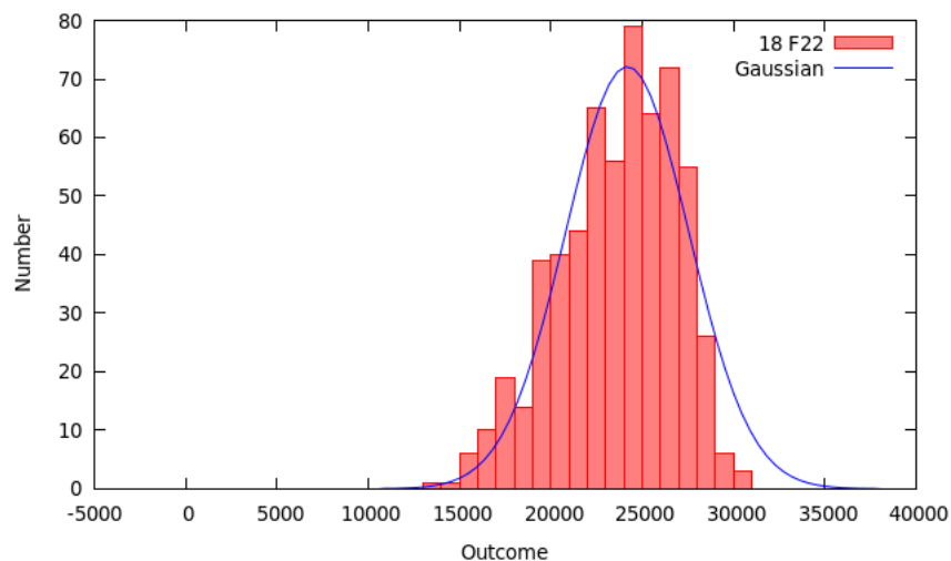
Figure 7.3 Histogram results curve fit with a gaussian distribution.
