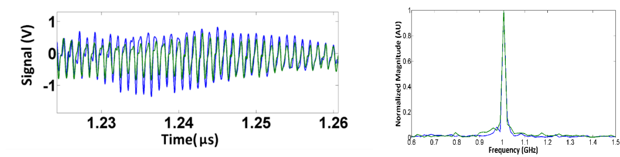
Figure 25: An example of a raw microwave signal produced by the RPM with the MCC-1 installed. Phase locking is evident (left), and the FFT (right) shows no indication of mode competition.
