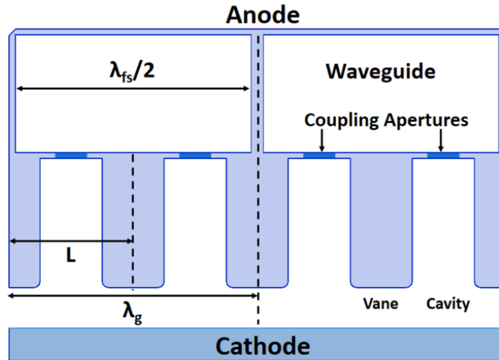
Figure 21: A 2D cross-section of an all-cavity extraction anode using standard rectangular waveguide on a planar RPM geometry.
