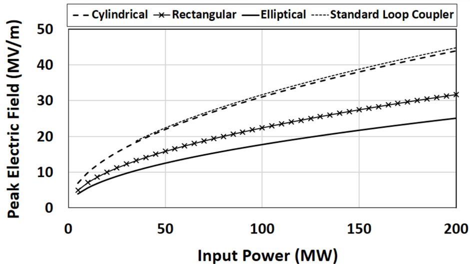
Figure 13: Peak electric field of each coupler design as a function of input power. The elliptical design, while complex to manufacture, demonstrates excellent performance.
