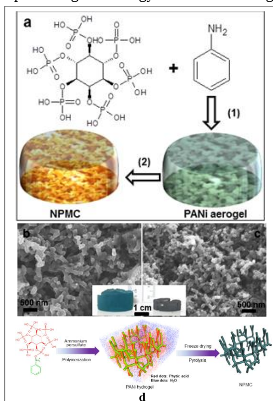
Figure 13. (a) Illustration of the preparation process of nitrogen and phosphorus co-doped porous carbon (NPMC) foams: (1) the formation of polyaniline (PANI) aerogel through an oxidative polymerization method; (2) pyrolysis of the PANi aerogel in Ar to produce NPMC. SEM images of (b) PANi aerogel and (c) NPMC-1000. Inset is the digital picture of PANi aerogel before (left) and after (right) pyrolysis at 1000 °C. (d) A schematic representation of the formation process of NPMC. (adapted from Nat. Nanotechnol. DOI:10.1038/nnano.2015.48, 2015.).
