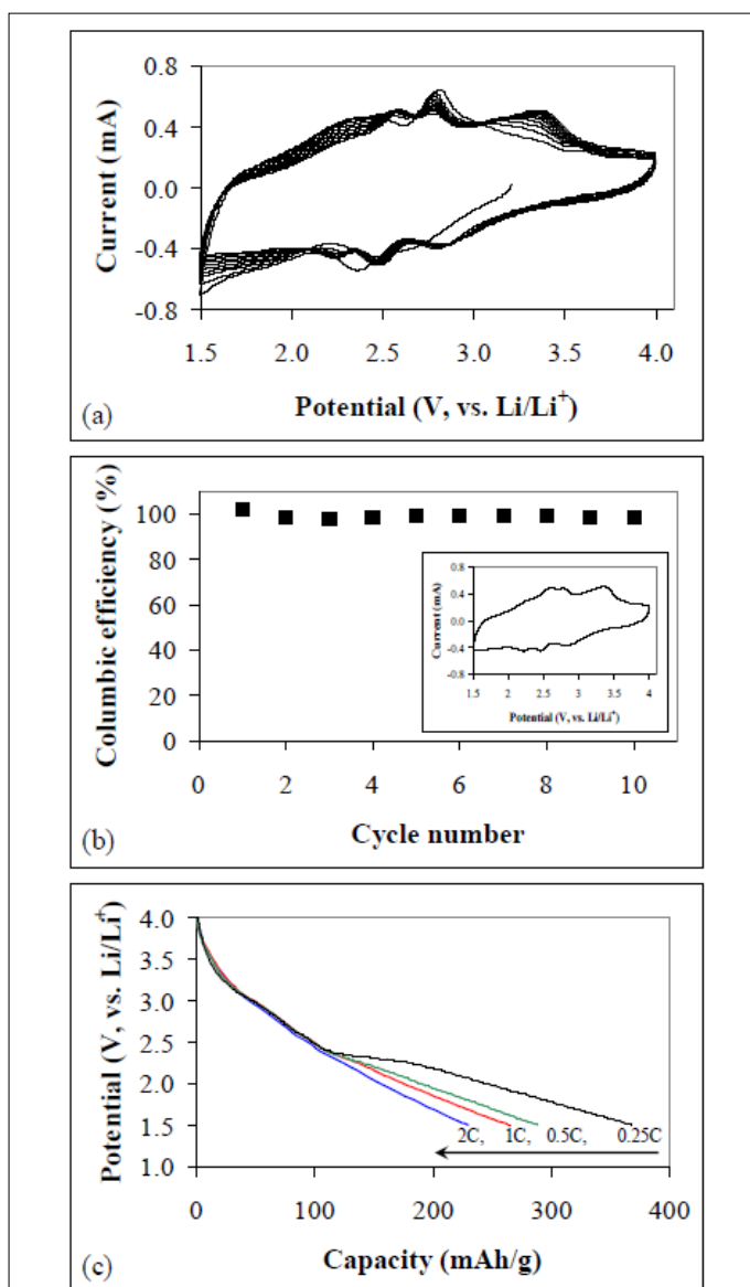
Figure 9. (a) CVs and (b) corresponding columbic efficiency of a \text{V}_2\text{O}_5 -VA-CNT electrode recorded in 1 M LiTFSI/20% EC/[EDMMEA][TFSI] electrolyte. Scan rate: 1 mV/s. The inset in (b) is the 10th cycle of the CV. (c) Discharge curves of the \text{V}_2\text{O}_5 -VA-CNT electrode recorded at the rates increasing from 0.25C to 2C as indicated by the arrow (curves shown were from the third cycle at each rate). Cut-off potential: 1.5 - 4 V. Galvanostatic charging/discharging (c) was performed for a same \text{V}_2\text{O}_5 -VA-CNT electrode after its CV test (a). (adapted from PhysChemChemPhys 2012, 14, 12099.).
