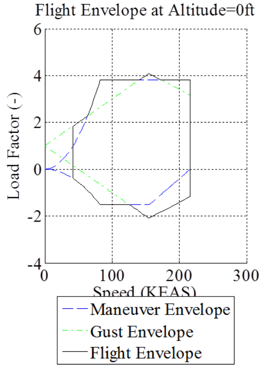
Figure 10: Flight envelope at an altitude of 0 feet.
