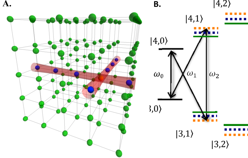
Figure 4: Addressing atoms in a 5 \times 5 \times 5 array. A.) Two circularly polarized laser beams pass through the lattice. The target atom sees twice the intensity of any other atom. The B-field is in the addressing beam plane at 45^\circ to the beams. B.) The addressing transitions in the Cs ground state hyperfine manifold (only partially shown here). Only the target atom is ac Stark shifted into resonance with the microwaves. It is transferred to the m_F=1 states, in which an arbitrary rotation on the Bloch sphere can be made. The target atom is then returned to the qubit states.
