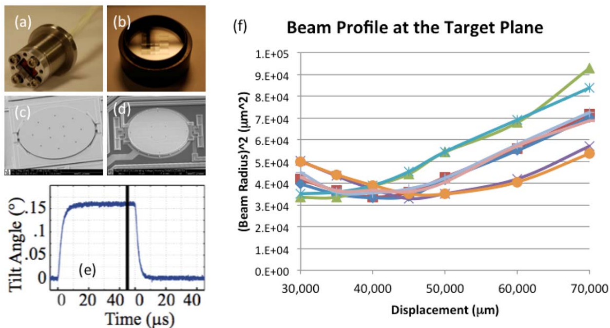
Figure 8: Components and performance of the initial 3D beam steering system. (a) Fiber array aligned with microlens array. (b) Lenslet array with different focal lengths that enables shift in focal points. (c, d) MEMS mirrors fabricated using the Sandia SUMMiT V process. (e) Switching speed for the initial MEMS mirrors. (f) Demonstration of the 3D focusing of the beams using the lenslet array.
