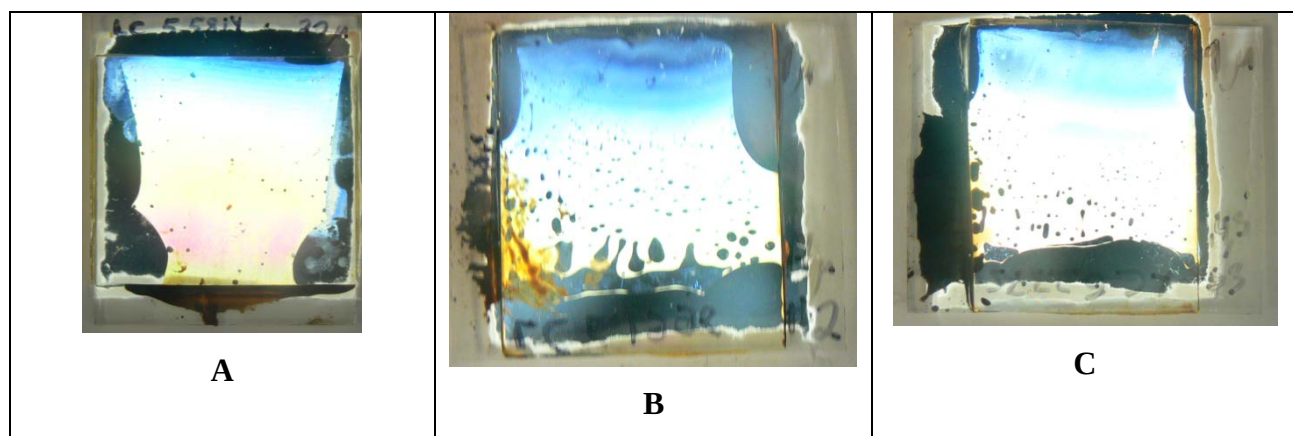
Figure 3. A: Photograph of wedge cell ( \beta = 1.45 mrad) filled with material VI cooled to \sim 22 °C. B: wedge cell ( \beta = 1.1 mrad) filled with material VII ; colorful horizontal stripes are seen in the upper part of the picture( T=230 °C - 190 °C). C: Wedge cell ( \beta = 1.0 mrad) filled with material V on cooling( T=190 °C - 160 °C); colorful horizontal stripes are seen in the upper part of the picture.
