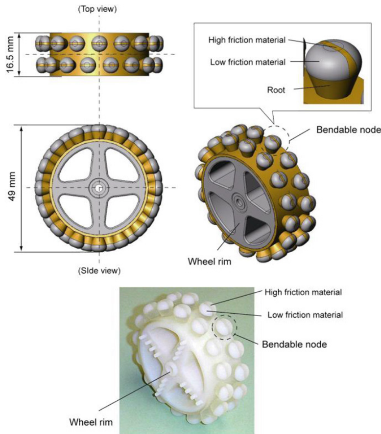
FIGURE 4 CAD model and prototype of the multi-material anisotropic friction wheel for omnidirectional vehicle.
