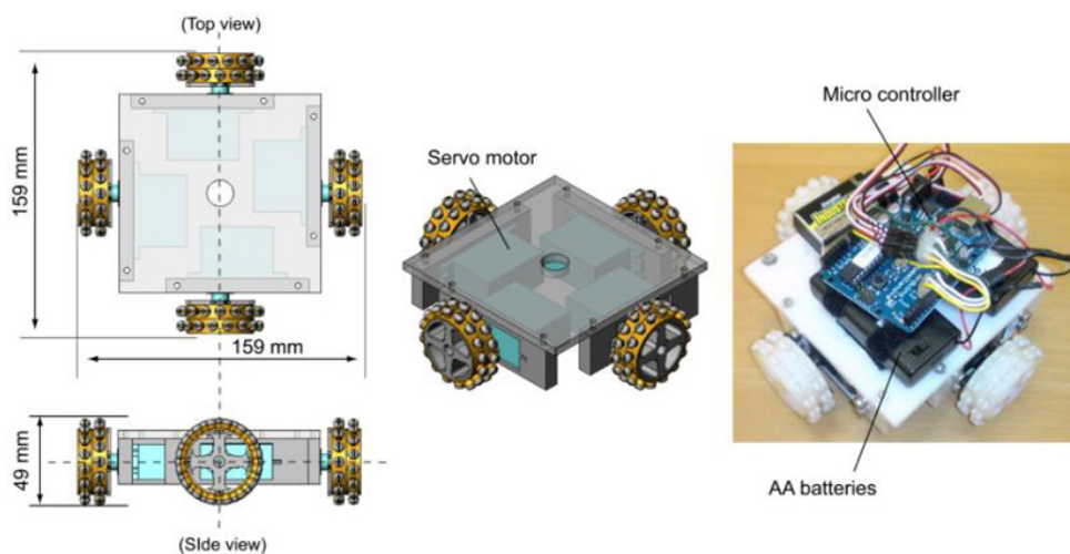
FIGURE 5 Prototype of the omnidirectional mobile with proposed wheel.
