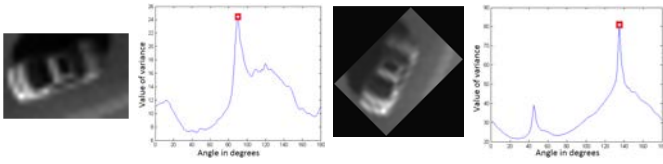
Fig. 3. Vehicle orientations are measured wrt vertical axis pointed up. (a) Car template. (b) Variance of Radon transform profiles with maximum at 90° (red sq). (c) Car template rotated by 45° CCW. (d) Peak in variance of Radon transform profiles at 135° (red sq), for correct change in orientation of 45°.
