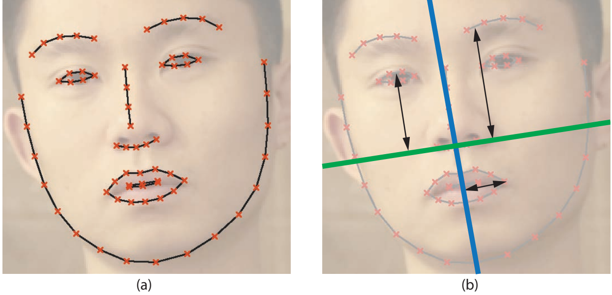
Figure 4.2: Facial features detected in a single video frame (a). We compute 2 axes per frame, a vertical line bisecting the face (blue) and a horizontal line across the base of the nose (green) (b). We measure facial regions by computing the perpendicular distance of their corresponding feature points to the axis perpendicular to their movement.
