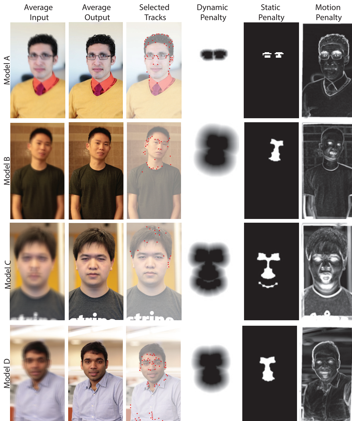
Figure 4.10: Notice that the average input images are blurry as there is camera shake, while the average output image is only blurry at facial features with movements. The automatically selected tracks lie on areas with no motion. The automatically generated penalties help to guide the composite to have motion only at moving facial parts and compositing seams should lie at regions with minimal appearance changes.
